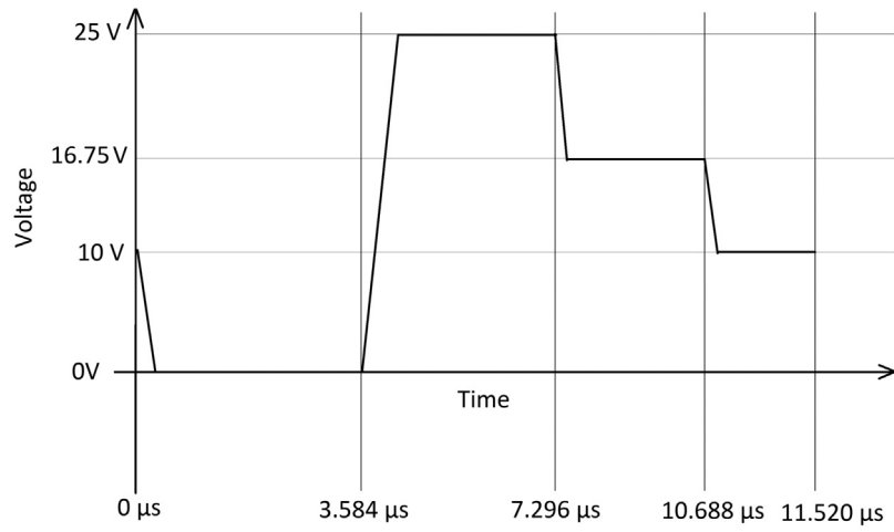
Fig. 2. Jetting waveform used perform printing on Dimatix.
