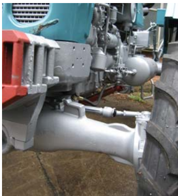
Slika 1. Novougrađeni pogonski most Figure 1. Newly installed drive axle
