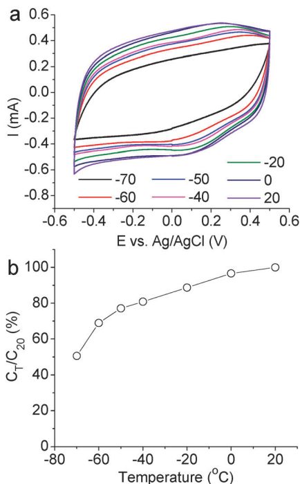
Fig. 2 (a) CVs and (b) C_7/C_{20} of a CNT electrode in the 2.0 \text{ mol L}^{-1} solution of \text{CaCl}_2 in mixed FA– \text{H}_2\text{O} (1 : 1 v : v) at different temperatures as indicated. Potential scan rate: 100 \text{ mV s}^{-1} .
