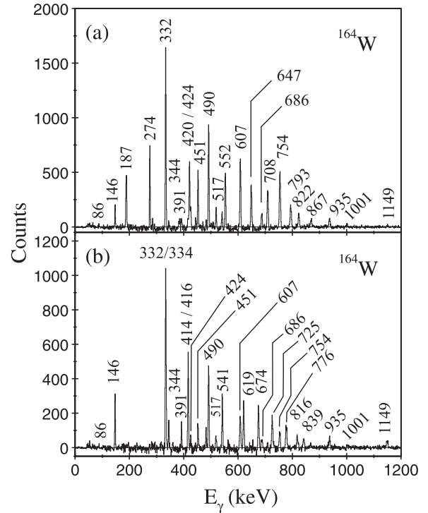
FIG. 3. \gamma -ray coincidences detected at the target position by the Jurogam spectrometer in delayed coincidence with recoils implanted in the DSSDs of the GREAT spectrometer located at the focal plane of the RITU separator. (a) Summed double-gated \gamma -ray spectrum generated by using a list of band-2 transitions comprising the 420, 552, 647, 708, 754, 793, and 822 keV transitions. (b) Summed double-gated \gamma -ray spectrum generated using a list of band-3 transitions comprising the 415, 541, 619, 674, 725, 776, and 816 keV transitions.
