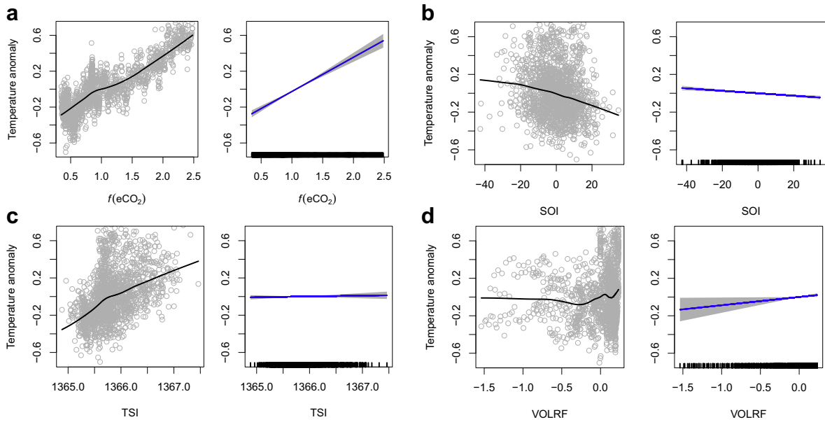
Fig. 4. Scatter plots and non-linear smooths of mean global temperature anomaly against the four covariates (left-hand figures in a–d). The lowess function in R ( http://www.r-project.org/ ) with default parameters was used to smooth these data. The right hand figures in a–d are the fitted spline curves from the gamm function in R using the same autocorrelation structure as Model A.
