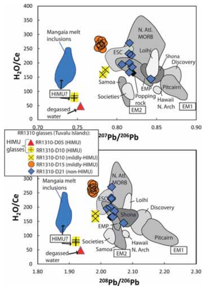
Figure 10. H_2O/Ce versus ^{208}Pb/^{206}Pb and ^{207}Pb/^{206}Pb for Tuvalu glasses and global OIBs and MORBs. Data from other OIB and MORB sources are provided for comparison and consist of submarine glass samples and melt inclusions [Staudigel et al., 1984; Hanan and Schilling, 1989; Devey et al., 1990; Dosso et al., 1991; Fontignie and Schilling, 1991; Woodhead and Devey, 1993; Douglass et al., 1995; Dixon, 1997; Kingsley and Schilling, 1998; Douglass et al., 1999; Dosso et al., 1999; Frey et al., 2000; Dixon and Clague, 2001; Dixon et al., 2002; Kingsley, 2002; Simons et al., 2002; Yang et al., 2003; Honda and Woodhead, 2005; Workman et al., 2006; Cartigny et al., 2008, and references therein; Hanyu et al., 2011; Kelley et al., 2013]. In both plots, the field for HIMU melt inclusions from Mangaia is defined by data published in Cabral et al. [2014], and excludes melt inclusions that have experienced diffusive H_2O -loss through the host olivine (i.e., all inclusions from sample MGA-B-47). The HIMU mantle reservoir is sampled by both Mangaia melt inclusions and by dredge 10 HIMU glasses from the Tuvalu. Dredge 5 glasses from the Tuvalu may have degassed significant H_2O by closed-system degassing processes. The figure is modified after Cabral et al. [2014], and methods for filtering the global database are provided in the same reference.
