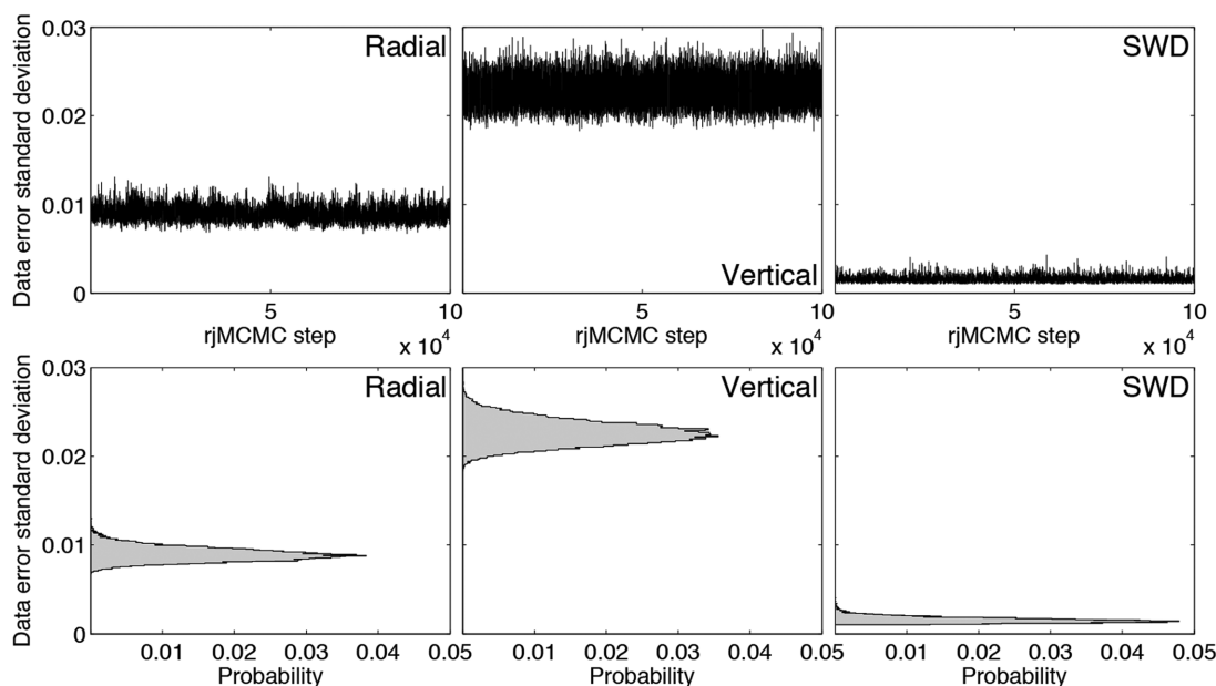
Figure 7. The standard deviation of the three independent data sets considered in the inversion of (a) radial and (b) vertical waveforms, and (c) SWD dispersion data. Note that no subjective choice is required to weight the individual data types.
