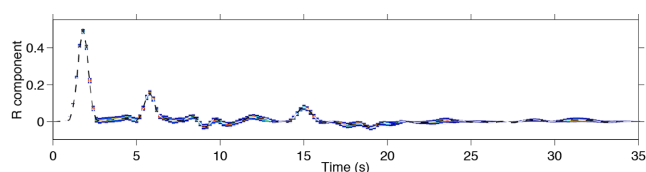
Figure 11. Observed RF (dashed) and range of data predictions (colour) for station HYB.
