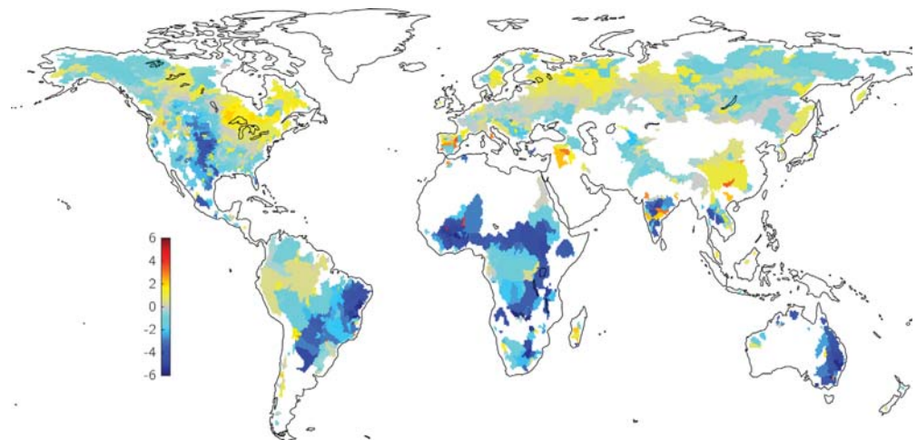
Figure 6. The difference in absolute square-root transformed QMEAN error between HBV with regionalized parameters (based on the 10 most similar donor catchments) versus spatially uniform parameters, using the observation-based QMEAN map of Beck [2016] as reference. Blue indicates HBV with regionalized parameters is closer to the observations, whereas yellow and red indicate HBV with spatially-uniform parameters is closer to the observations. White indicates that no observations were available. WFDEI precipitation was used to drive HBV.
