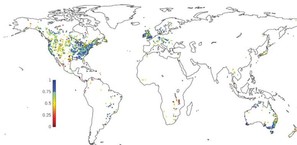
Figure 2. The minimum values of the calibration and validation AOF scores obtained using HBV for the study catchments. Each data point represents a catchment centroid ( n = 1787 ). Catchments indicated in blue obtained calibration and validation scores > 0.75 and were used as donor catchment for the regionalization scheme. CPC precipitation was used to drive the model.
