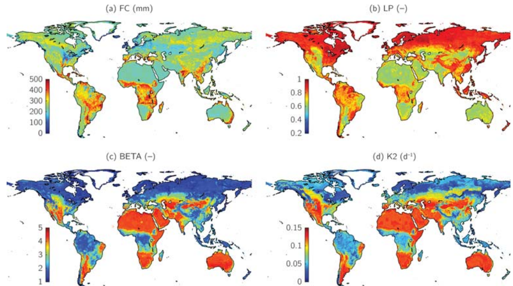
Figure 4. For HBV, mean values of the regionalized parameters based on the 10 most similar donor catchments for: (a) the maximum water storage in the unsaturated-zone store (FC); (b) the soil moisture value above which actual evaporation reaches potential evaporation (LP); (c) the shape coefficient of recharge function (BETA); and (d) the recession coefficient of lower groundwater store (K2). For maps of all other parameters, see supporting information Figure S2.1.
