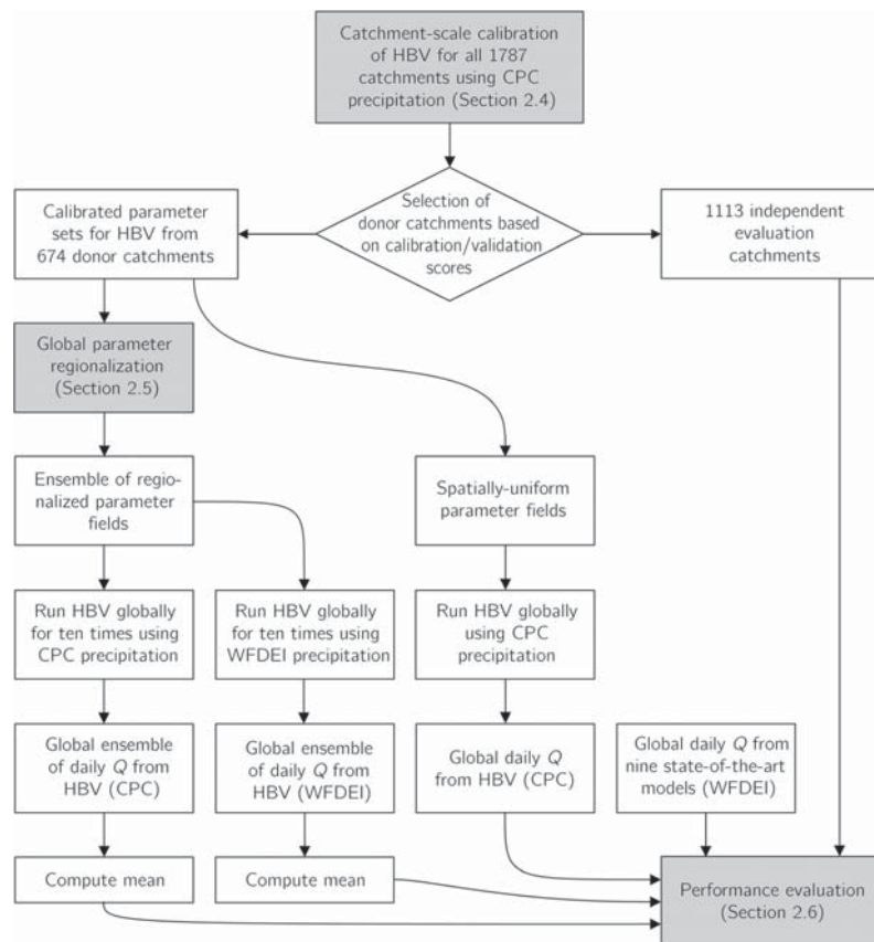
Figure 1. Flow chart summarizing the various steps carried out in this study to implement and test the regionalization scheme.
