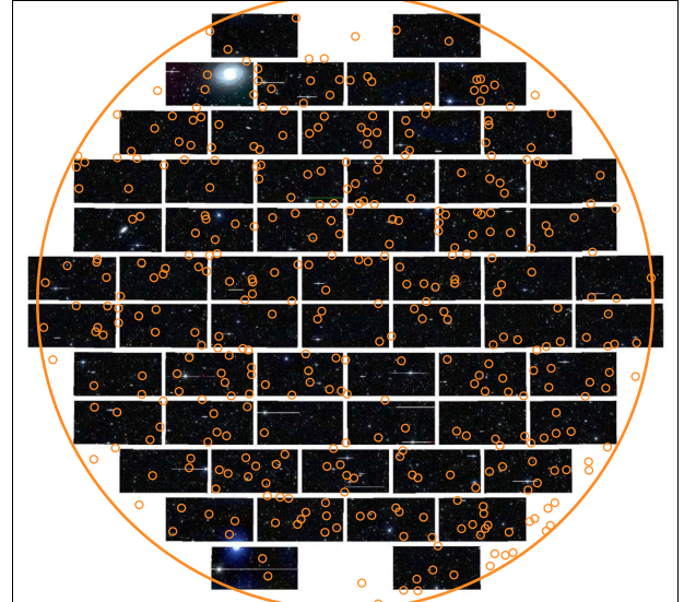
Figure 1. The 2dF spectrograph has 392 optical fibres to be placed at positions across a field of view 2^\circ 1 in diameter (large orange circle). This is well matched to the DECam field of view (image mosaic in the background), making spectroscopic follow-up very efficient. The small orange circles represent the locations of targets selected for one set of AAT observations.
