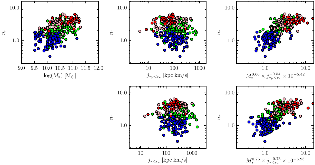
Figure 4. Projections of the M_*-j_*-n_r plane. The top row shows, from left to right, the M_*-n_r , j_{*p}<r_e-n_r , and the projection that minimizes the scatter in n_r . The bottom row is the same as the top row, but for the intrinsic j_* . Symbols are colour-coded by morphological type as in Fig. 2.
