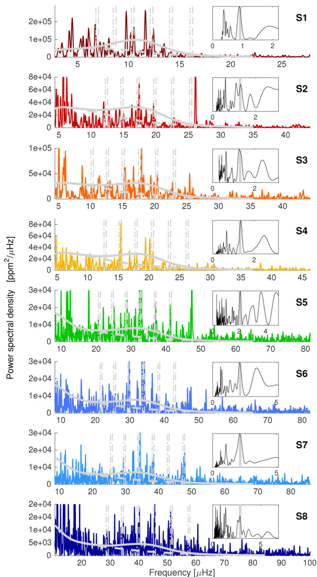
Figure 2. Solar-like oscillation spectra of eight K giants observed by K2. The bottom star is in the RHB. Stars (from top to bottom) are ordered by increasing \nu_{\text{max}} . Vertical lines show the position of radial (dashed lines) and quadrupole (dash–dotted lines) oscillation frequencies as expected by the pattern of oscillation modes in red-giant stars described in Mosser et al. (2011). The expected granulation power and the combined granulation and oscillation power are represented by dashed and solid thick lines. The insets show the power spectrum of the power spectrum (PSPS) of each star, computed from the region around \nu_{\text{max}} . In each PSPS, the prominent peak at \Delta\nu/2 (vertical grey line) is the detected signature of the near-regular spacing of oscillation peaks in the frequency spectrum.
