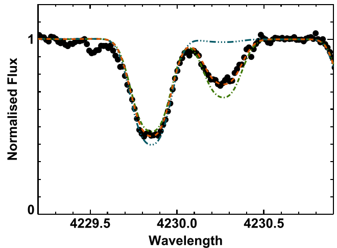
Figure 3. Synthesis of the ^{13}\text{C}\text{H} line at 4230 Å in HE 2208–1239 for three different isotopic ratios; 100% ^{12}\text{C}\text{H} (blue), ^{12}\text{C}/^{13}\text{C} = 79/21 (red), and ^{12}\text{C}/^{13}\text{C} = 70/30 (green).
