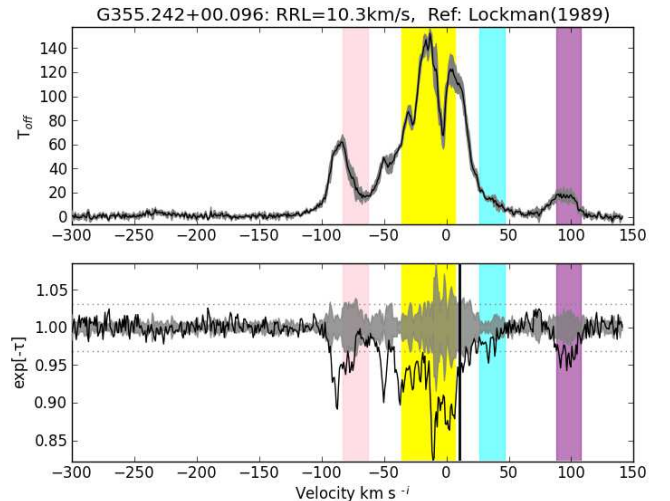
FIG. 1.— Figure Set: H I emission/absorption spectrum pairs. In each figure, the top panel shows the emission spectra. The emission is shown by the solid line (this is the average of the three ‘off’ positions, see 3.1) and the emission envelope (difference between the ‘off’ positions) is shown in grey. Absorption, e^{-\tau} , is displayed in the bottom panel. The H I absorption spectrum (see 2) is shown by the solid line and the grey envelope signifies 3\sigma_{e^{-\tau}} (calculated from the emission envelope, see §3). The absorption panel also displays the RRL velocities of the H II region (solid vertical lines) and the fluctuation in the baseline of the absorption spectrum ( 3\sigma_{rms_{e^{-\tau}}} ) (horizontal dotted lines). The H II region name, RRL velocity and reference are shown as well as the expected velocity ranges of EIG features (see §4.1) with the same color system as Figure 2.
