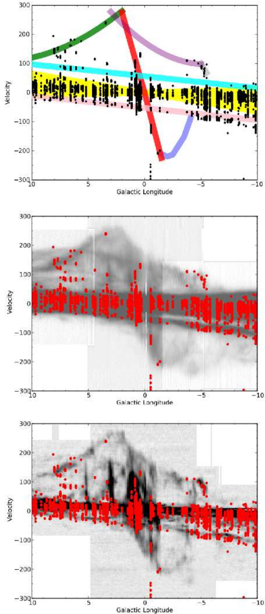
FIG. 3.— lv diagrams showing velocity channels with significant absorption for each H II region overlaid onto: top panel - the ‘crayon’ plot of EIG features (see Figure 2); middle panel - H I emission (the intensity map was created from the SGPS I & II and ATCA HIGCS); bottom panel - CO emission (see Figure 2). (A color version of this figure is available in the online journal.)
