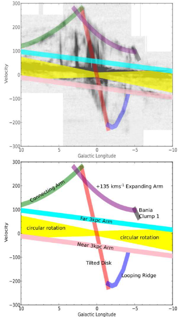
FIG. 2.— Longitude-velocity ‘crayon’ diagram for l < |10^\circ| , b < |1.5^\circ| . Top panel - the ‘crayon’ features overlaid on CO emission map (Dame et al. 2001). Bottom panel - the ‘crayon’ features (each with a velocity width of 20\text{ km s}^{-1} ). The ‘crayon’ color system is as follows: yellow - circular rotation allowed velocity envelope; green - Connecting Arm; purple - +135\text{ km s}^{-1} Expanding Arm; grey - Bania’s Clump 1; red - Tilted Disk; cyan - Far 3kpc Arm; yellow - velocities allowed by circular disk rotation; pink - Near 3kpc Arm; blue - Looping Ridge. While not explicitly labeled in the crayon diagram, Bania’s Clump 2 can be seen as the thick vertical CO feature at l \sim 3^\circ , 0 \lesssim v \lesssim 200\text{ km s}^{-1} in the top panel. (A color version of this figure is available in the online journal.)
