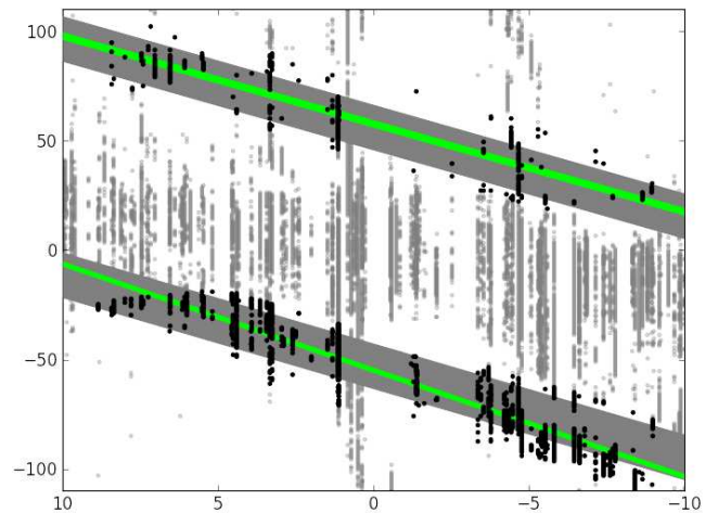
FIG. 4.— Velocity channels of significant H I absorption: those included in the tracing of the 3kpc Arms are shown in black, while those channels which were excluded from the analysis are in grey. The fits of Dame & Thaddeus (2008) are given by the grey bands (see Figure 2), the fits from this analysis are displayed in green. (A color version of this figure is available in the online journal.)
