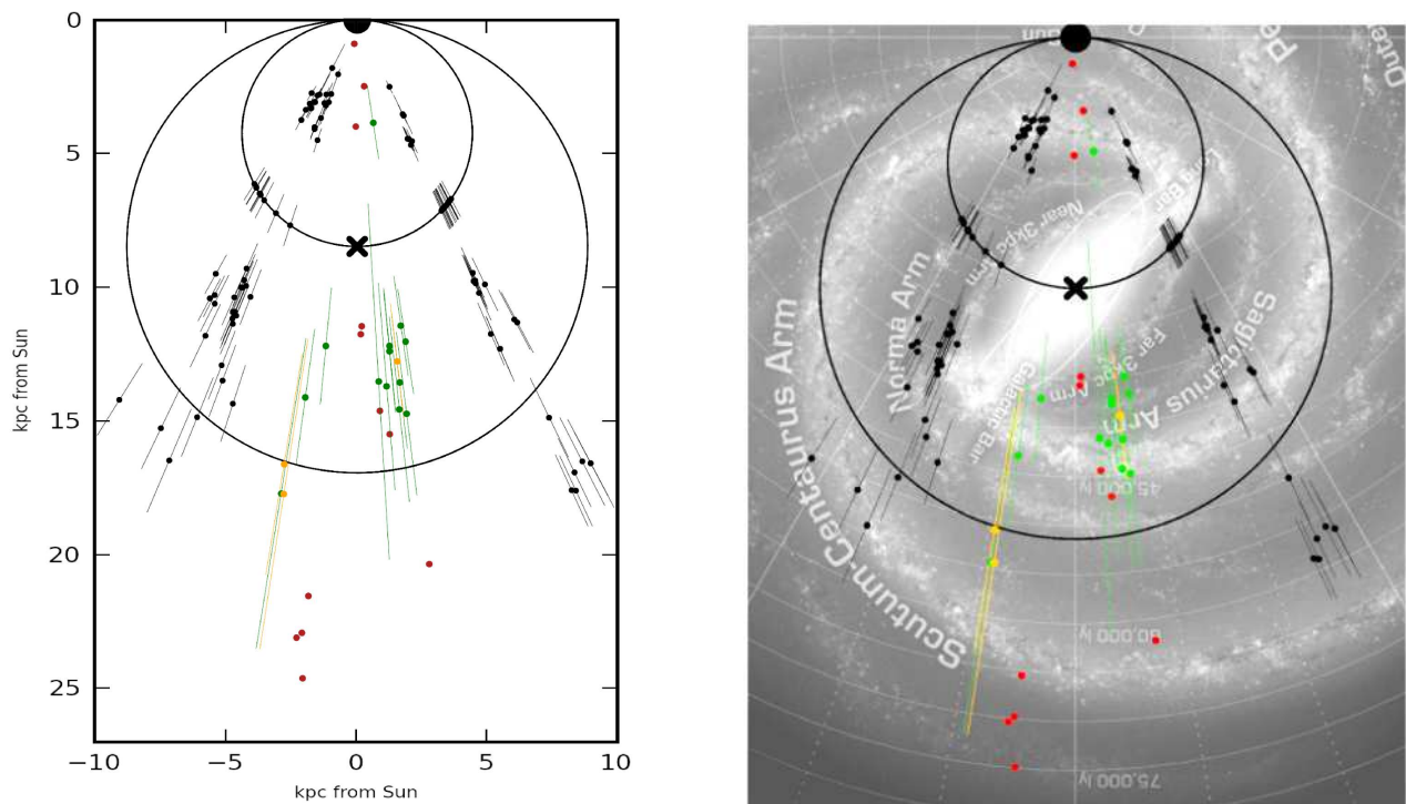
FIG. 7.— Positions of the H II region complexes for which a kinematic distance was calculated (Quality A, B and C shown as green, orange and red markers respectively). Also shown are the Solar Circle and locus of tangent points (black circles) and kinematic distances for H II regions from Jones & Dickey (2012) (black markers). Error bars are calculated according to the analysis of §7.1.1; the large uncertainties are not shown for quality C distances. Background image credit [right panel]: Hurt & Benjamin in Churchwell et al. (2009). (A color version of this figure is available in the online journal.)
