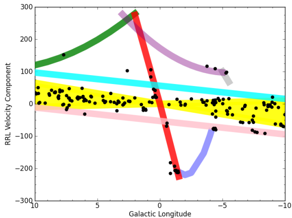
FIG. 5.— Longitude-velocity ‘crayon’ diagram (see Figure 2) showing the distribution of H II region RRL velocity components. (A color version of this figure is available in the online journal.)
