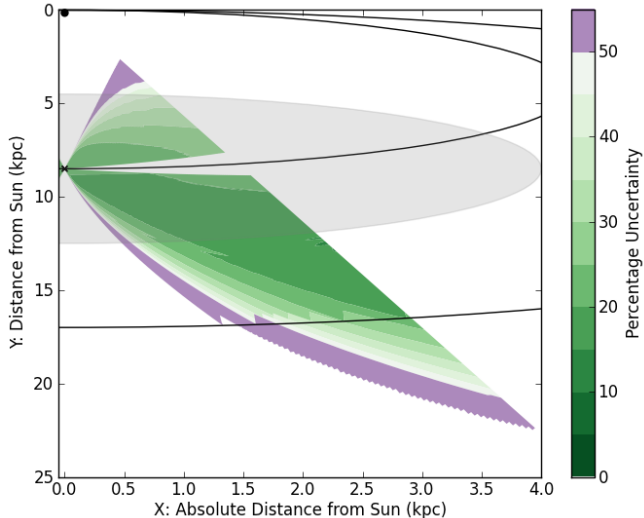
FIG. 6.— Total percentage uncertainty in the line of sight distance D_{los} caused by the choice of rotation curve, non-circular streaming motions of 15\text{ km s}^{-1} and by changing the Solar circular rotation speed to \Theta_o = 255\text{ km s}^{-1} . Blank areas are indicative of |l| > 10^\circ (where no error analysis was carried out), or percentage uncertainties > 100\% . The EIG is shaded grey (no kinematic distances were calculated for this region), and the Solar Circle and Locus of Tangent Points appear as the black circles. The percentage uncertainties are mirrored for lines of sight in the fourth quadrant, here, only l > 0 is shown for clarity. (A color version of this figure is available in the online journal.)
