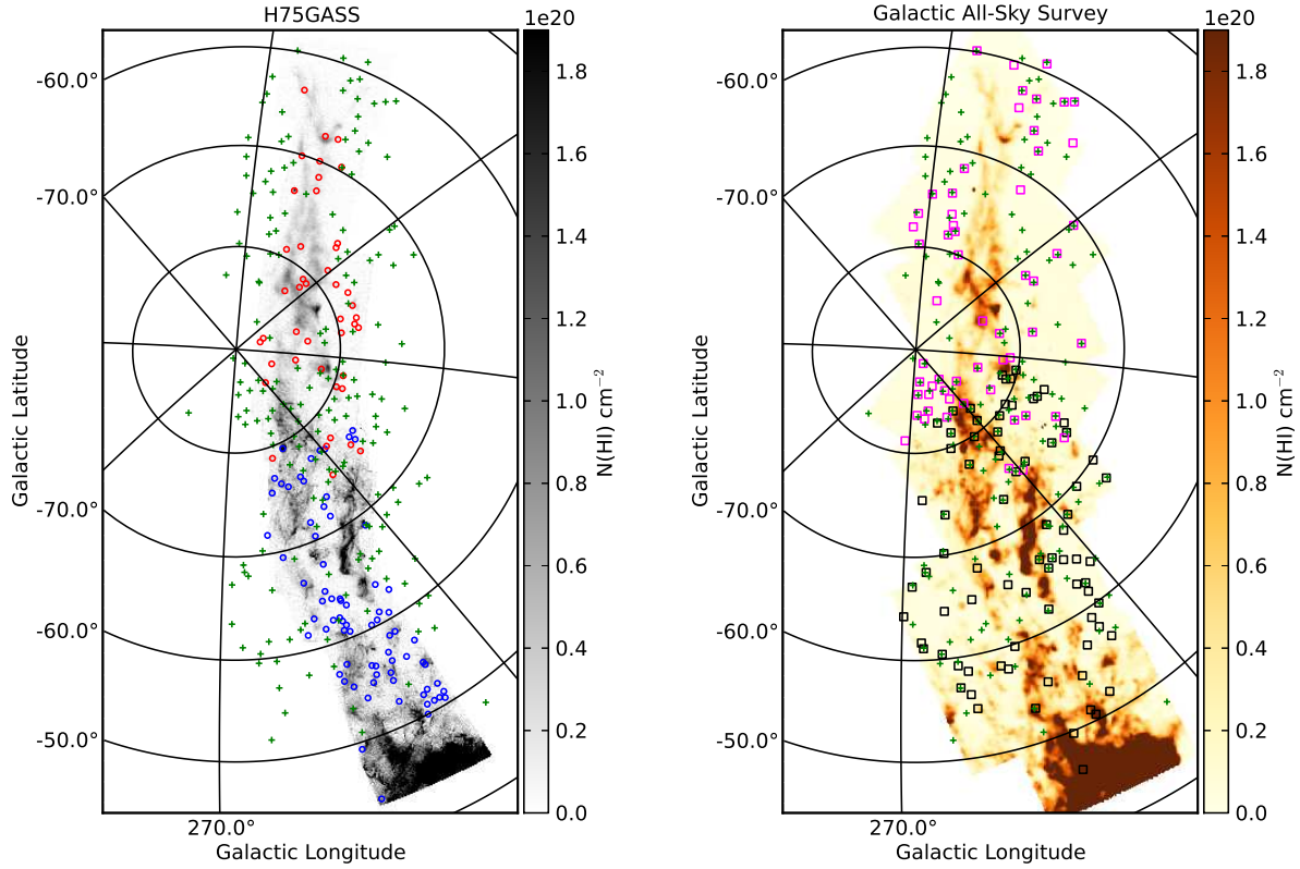
Fig. 5.— Left : All 118 sources detected by Duchamp with the H75GASS data (red and blue circles) and 183 sources detected by Putman et al. (2002) (green pluses) are overlaid onto the integrated HI column density map of H75GASS as shown in Figure 1. The blue and red circles represent Duchamp detections at positive and negative LSR velocities, respectively. Right : Same as left figure, except 135 sources detected by Duchamp are from GASS data and are overlaid onto the HI column density map of GASS as shown in Figure 2. The black and magenta squares represent Duchamp detections at positive and negative LSR velocities, respectively. The sources from Putman et al. (2002) are within the same V_{\text{LSR}} range and the same region on the sky as our GASS data presented in this paper.
