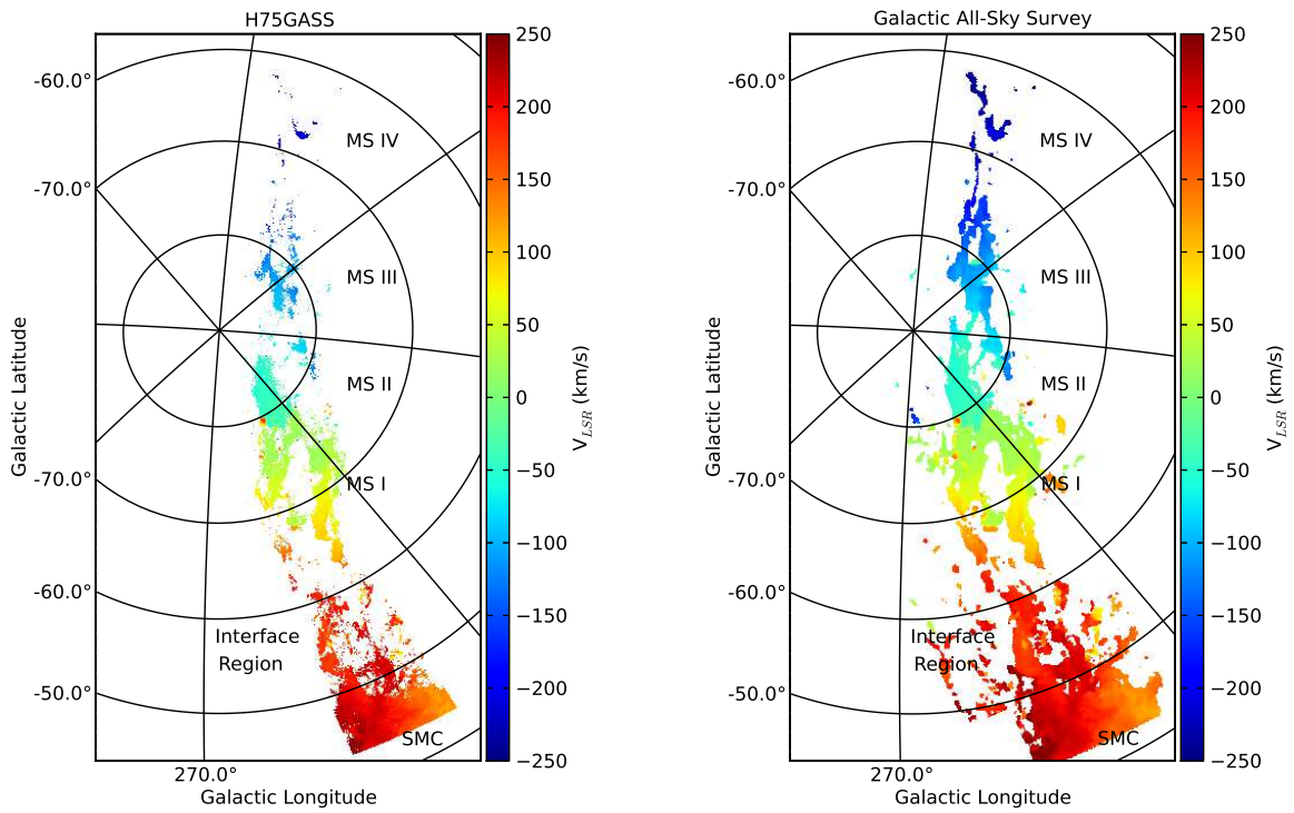
Fig. 10.— Velocity field map in the LSR frame with a velocity range from -250 to +250 \text{km s}^{-1} for H75GASS (left) and GASS (right). The Small Magellanic Cloud, the Interface Region, and MS I–IV are labeled.
