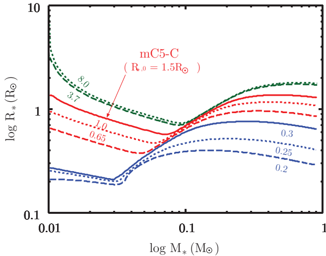
Figure 5. Same as Figure 2 but for cases with different initial radii: R_{*,0} = 8.0 R_{\odot} (green dotted, case mC5-C-Ri8), R_{*,0} = 3.7 R_{\odot} (green dashed, case mC5-C-Ri3.7), R_{*,0} = 1.5 R_{\odot} (red solid, case mC5-C), 1.0 R_{\odot} (red dotted, case mC5-C-Ri1), 0.65 R_{\odot} (red dashed, case mC5-C-Ri0.65), 0.3 R_{\odot} (blue solid, case mC5-C-Ri0.3), 0.25 R_{\odot} (blue dotted, case mC5-C-Ri0.25), and 0.2 R_{\odot} (blue dashed, case mC5-C-Ri0.2). The values of the initial radii are labeled in the panel. The cold mass accretion at the constant rate \dot{M} = 10^{-5} M_{\odot} \text{ yr}^{-1} is adopted for all the cases.
