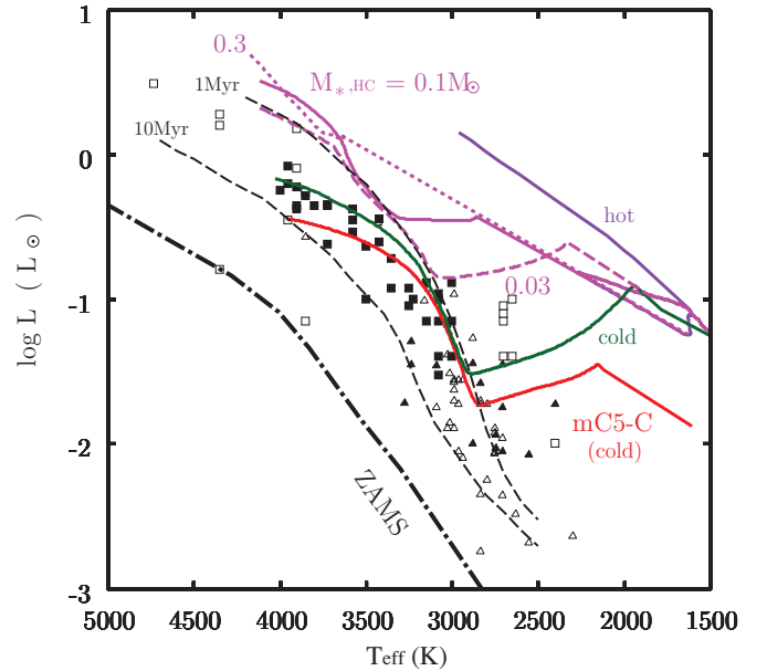
Figure 9. Same as Figure 6 but for varying the thermal efficiency of mass accretion. Different lines indicate the different thermal efficiencies: only hot mass accretion (purple, case mC5-H), cold accretion followed by early hot accretion for M_* < M_{*,\text{HC}} = 0.3 M_{\odot} (magenta dotted, case mC5-HC0.3), 0.1 M_{\odot} (magenta solid, case mC5-HC0.1), 0.03 M_{\odot} (magenta dashed, case mC5-HC0.03), and only cold mass accretion with the same initial model as in the above cases (green, case mC5-C-Ri3.7).
