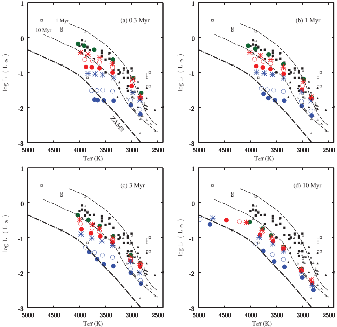
Figure 7. Same as Figure 3 but for the cases presented in Figure 6 and for the PMS stars of various masses. The symbols in each panel mark the positions of 0.9 M_{\odot} , 0.7 M_{\odot} , 0.5 M_{\odot} , 0.3 M_{\odot} , 0.1 M_{\odot} , and 0.05 M_{\odot} stars from the left for cases mC5-C-Ri3.7 (green filled circles), mC5-C (red asterisks), mC5-C-Ri1 (red open circles), mC5-C-Ri0.65 (red filled circles), mC5-C-Ri0.3 (blue asterisks), mC5-C-Ri0.25 (blue open circles), and mC5-C-Ri0.2 (blue filled circles). We omit the evolutionary tracks for clarity here. We also omit model mC5-C-Ri8 because it is nearly identical to mC5-C-Ri3.7.
