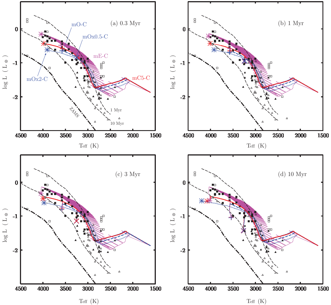
Figure 3. Snapshots of stellar positions in the HRD for varying accretion histories with the same initial and boundary conditions. The four panels show the snapshots at times 0.3 Myr (a), 1 Myr (b), 3 Myr (c), and 10 Myr (d) after the start of mass accretion. The evolutionary tracks until that time are also plotted in the panels. (Note that the luminosity plotted here is only the stellar luminosity; accretion luminosity is not included.) The different colors represent different accretion histories: constant accretion at 10^{-5} M_{\odot} \text{ yr}^{-1} (red, case mC5-C), episodic accretion (magenta, case mE-C), and decreasing accretion (blue, cases mO-C, mOx2-C, mOx0.5-C). The input parameters in each case are summarized in Table 1a. In each panel, the symbols mark the positions of stars whose masses are 0.9 M_{\odot} (asterisks), 0.45 M_{\odot} (pluses), and 0.23 M_{\odot} (crosses). The thick dot-solid line indicates the positions of ZAMS stars (Siess et al. 2000). The dashed lines represent the isochrones of 1 Myr and 10 Myr for non-accreting protostars (Baraffe et al. 1998). Observational data are taken from Gatti et al. (2006, open squares), Gatti et al. (2008, filled squares), Muzerolle et al. (2005, open triangles), and Peterson et al. (2008, filled triangles). (A color version of this figure is available in the online journal.)
