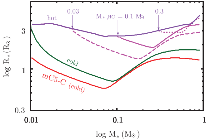
Figure 8. Same as Figure 2 but for cases with different thermal efficiencies of mass accretion. Only hot and cold mass accretion is adopted with the same initial radius 3.7 R_{\odot} in cases mC5-H (purple) and mC5-C-Ri3.7 (green). In the cases with the magenta lines, the hot mass accretion is switched to the cold accretion when the stellar mass reaches M_{*,\text{HC}} = 0.3 M_{\odot} (magenta dotted, case mC5-HC0.3), 0.1 M_{\odot} (magenta solid, case mC5-HC0.1), and 0.03 M_{\odot} (magenta dashed, case mC5-HC0.03). The values of M_{*,\text{HC}} are labeled in the figure. The input parameters for these models are summarized in Table 1c. The red line represents the evolution in case mC5-C for a comparison.
