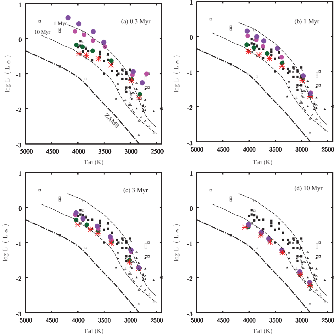
Figure 10. Same as Figure 7 but for the cases presented in Figure 9. The symbols in each panel mark the positions of 0.9 M_{\odot} , 0.7 M_{\odot} , 0.5 M_{\odot} , 0.3 M_{\odot} , 0.1 M_{\odot} , and 0.05 M_{\odot} stars from the left for cases mC5-H (purple filled circles), mC5-HC0.03 (magenta filled circles), mC5-C-Ri3.7 (green filled circles), and mC5-C (red asterisks).
