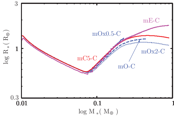
Figure 2. Evolution of the stellar radius vs. stellar mass for cases mC5-C (red), mE-C (magenta), mOx0.5-C (blue solid), mO-C (blue dashed), and mOx2-C (blue dotted), among which the accretion histories differ but the initial and boundary conditions do not.
