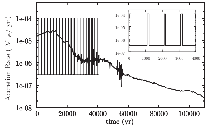
Figure 1. Time-dependent accretion histories adopted for calculations of protostellar evolution. The thick solid line presents the sample accretion history taken from the numerical simulations of low-mass star formation by Offner et al. (2009) and used in model mO-C. The thin solid line shows the vigorous episodic accretion case used in model mE-C, where a burst-like accretion phase at 10^{-4} M_{\odot} \text{ yr}^{-1} over 100 years is interspersed with a quiescent phase at 3 \times 10^{-7} M_{\odot} \text{ yr}^{-1} over 1000 years. The accretion history over initial 40,000 years is shown for this case. The small window enlarges the evolution over the initial 4000 years.
