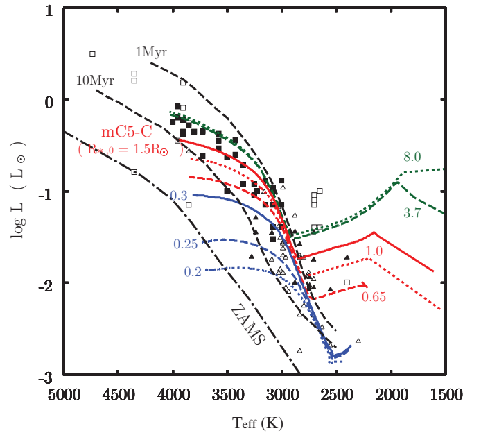
Figure 6. Evolution tracks with varying the initial radius with the cold mass accretion. The constant accretion rate of 10^{-5} M_{\odot} \text{ yr}^{-1} is adopted for these all cases. The tracks until the protostellar mass reaches 0.9 M_{\odot} by mass accretion are presented. The different lines show the evolution with different initial radii: R_{*,0} = 8.0 R_{\odot} (green dotted, case mC5-C-Ri8), R_{*,0} = 3.7 R_{\odot} (green dashed, case mC5-C-Ri3.7), R_{*,0} = 1.5 R_{\odot} (red solid, case mC5-C), 1.0 R_{\odot} (red dotted, case mC5-C-Ri1), 0.65 R_{\odot} (red dashed, case mC5-C-Ri0.65), 0.3 R_{\odot} (blue solid, case mC5-C-Ri0.3), 0.25 R_{\odot} (blue dotted, case mC5-C-Ri0.25), and 0.2 R_{\odot} (blue dashed, case mC5-C-Ri0.2). The initial radius in each model is labeled in the figure. The input parameters for these models are summarized in Table 1b.
