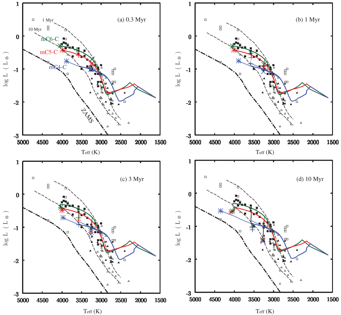
Figure 4. Same as Figure 3 but for different constant accretion rates. The different colors donate differences of the accretion rates: 10^{-6} M_{\odot} \text{ yr}^{-1} (green, case mC6-C), 10^{-5} M_{\odot} \text{ yr}^{-1} (red, case mC5-C), and 10^{-4} M_{\odot} \text{ yr}^{-1} (blue, case mC4-C). Parameters in each case are summarized in Table 1a.
