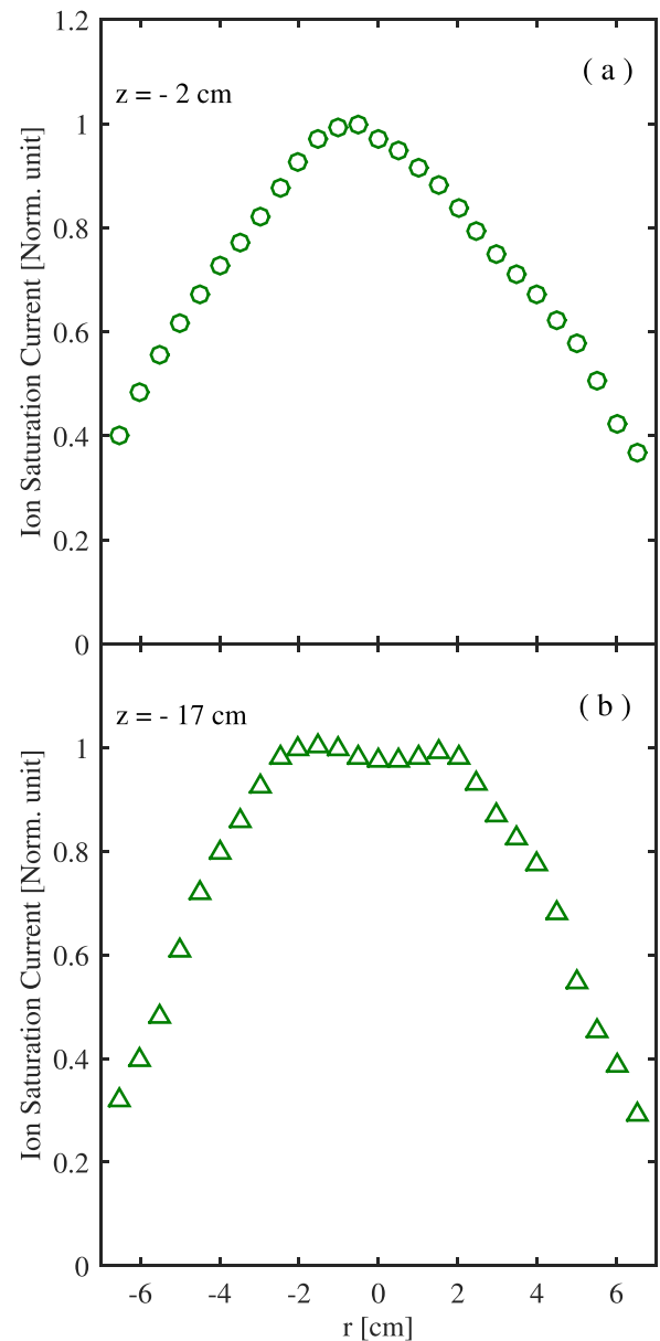
FIG. 4. Radial profiles of normalized ion saturation current measured by the LP at, (a) z = -2 cm in the source-exit region (○) and (b) z = -17 cm in the source-top region (△).
