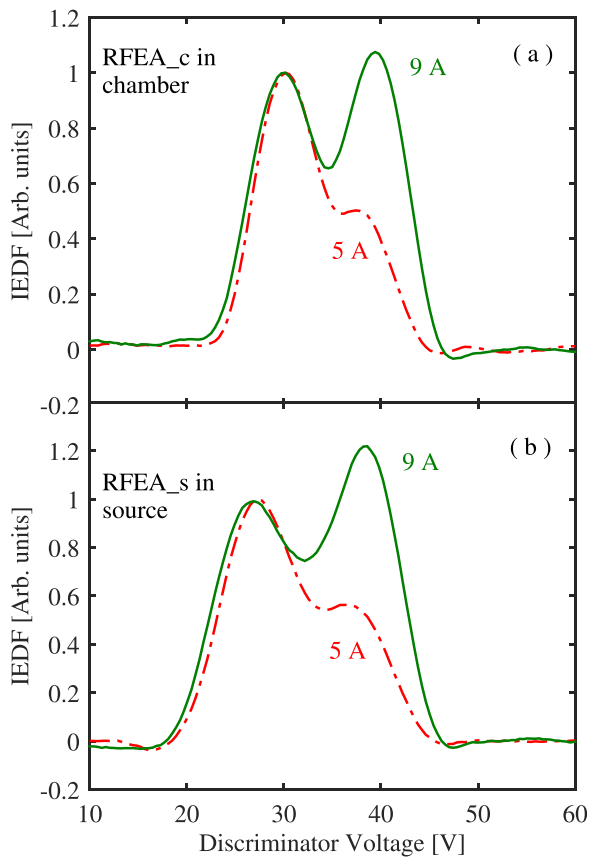
FIG. 3. IEDFs obtained by (a) RFEA_c at z = 7 cm in the diffusion chamber and (b) RFEA_s at z = -25 cm in the plasma source, for current values of 9 A (solid line) and 5 A (dashed-dotted line) supplied into the solenoid.
