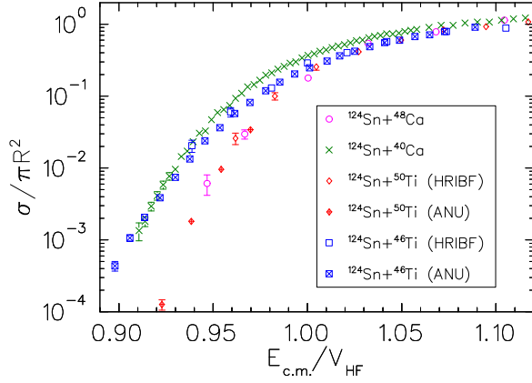
FIG. 6. Comparison of the reduced fusion excitation functions for ^{40}\text{Ca} + ^{124}\text{Sn} [7], ^{48}\text{Ca} + ^{124}\text{Sn} [5], ^{50}\text{Ti} + ^{124}\text{Sn} , and ^{46}\text{Ti} + ^{124}\text{Sn} .
