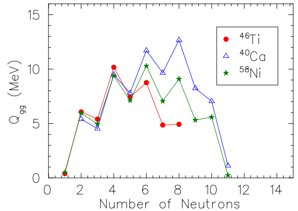
FIG. 1. Ground-state Q values as a function of the number of neutrons picked up by ^{46}\text{Ti} , ^{40}\text{Ca} , and ^{58}\text{Ni} from ^{124}\text{Sn} . Only the channels with positive Q values are shown.
