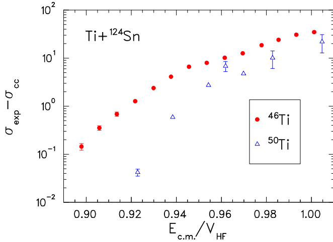
FIG. 3. Fusion excitation functions calculated by CCFULL subtracted from those measured for ^{46}\text{Ti} + ^{124}\text{Sn} and ^{50}\text{Ti} + ^{124}\text{Sn} .
