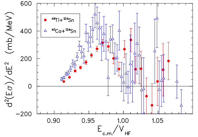
FIG. 7. Comparison of barrier distributions for ^{40}\text{Ca} + ^{124}\text{Sn} [7] and ^{46}\text{Ti} + ^{124}\text{Sn} obtained from the measured fusion excitation functions.
