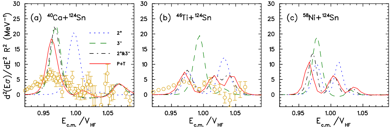
FIG. 8. Reduced barrier distributions for (a) ^{40}\text{Ca} + ^{124}\text{Sn} , (b) ^{46}\text{Ti} + ^{124}\text{Sn} , and (c) ^{58}\text{Ni} + ^{124}\text{Sn} , calculated by the coupled-channel code CCFULL. The results of coupled-channel calculations including inelastic excitations of the projectile are shown by the broken curves and inelastic excitations of both the projectile and target are shown by the solid curves. The experimental data are shown by the open circles.
