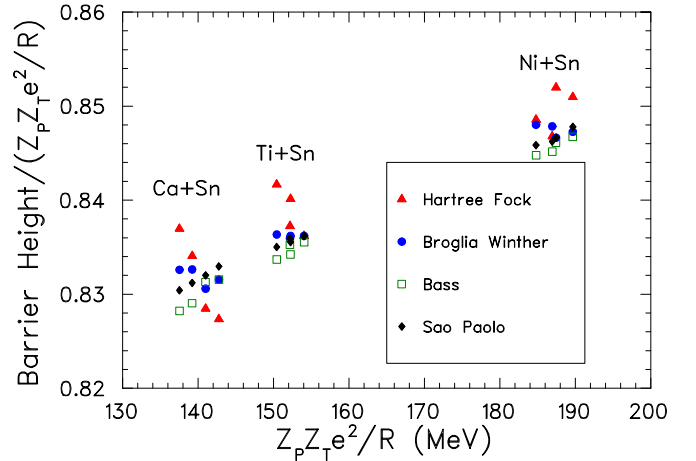
FIG. 4. Reduced barrier heights predicted by the frozen Hartree-Fock method, Broglia-Winther systematics, the Bass model, and the Sao Paulo model as a function of Z_P Z_T e^2 / R for ^{40,48}\text{Ca} + ^{124,132}\text{Sn} , ^{46,50}\text{Ti} + ^{124,132}\text{Sn} , and ^{58,64}\text{Ni} + ^{124,132}\text{Sn} .
