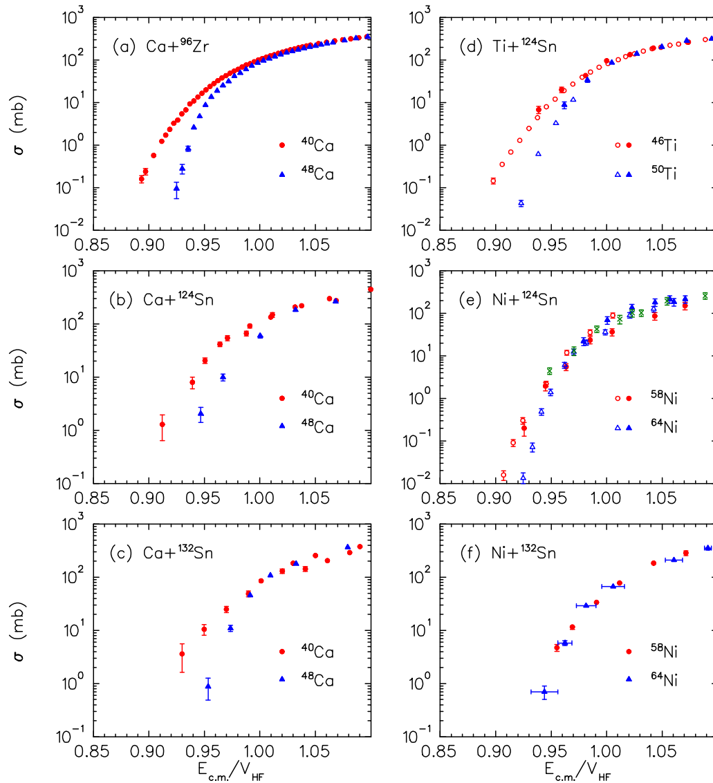
FIG. 5. Comparisons of reduced fusion excitation functions for (a) ^{40,48}\text{Ca} + ^{96}\text{Zr} , (b) ^{40,48}\text{Ca} + ^{124}\text{Sn} , (c) ^{40,48}\text{Ca} + ^{132}\text{Sn} , (d) ^{46,50}\text{Ti} + ^{124}\text{Sn} , (e) ^{58,64}\text{Ni} + ^{124}\text{Sn} , and (f) ^{58,64}\text{Ni} + ^{132}\text{Sn} . The data points shown by the crosses in (e) are for ^{64}\text{Ni} + ^{118}\text{Sn} . The reduced energy is obtained by dividing the center-of-mass energy by the barrier height predicted by the frozen HF method.
