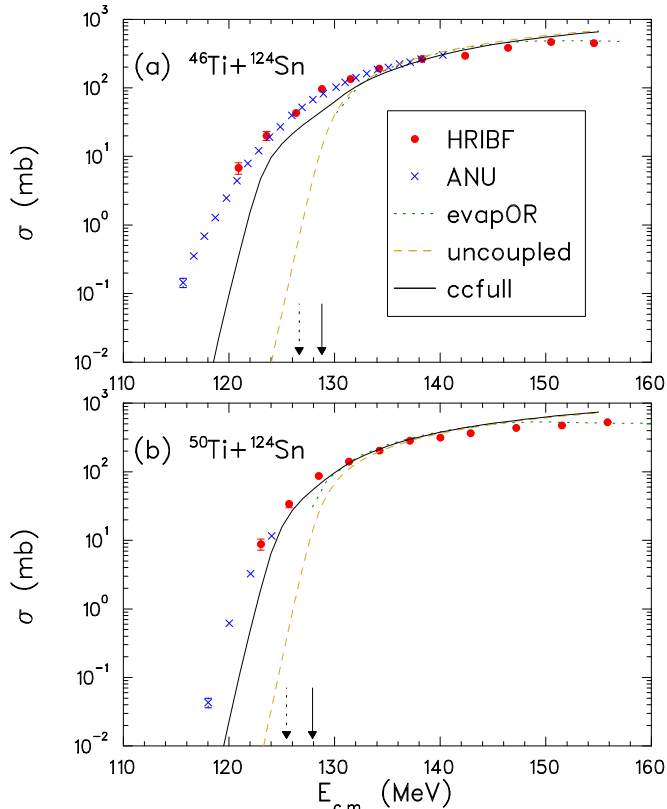
FIG. 2. Fusion excitation functions for (a) ^{46}\text{Ti} + ^{124}\text{Sn} and (b) ^{50}\text{Ti} + ^{124}\text{Sn} . The measurements were performed in inverse kinematics at HRIBF and in normal kinematics at ANU. Also shown are the ER cross sections predicted by the statistical model code EVAPOR, the results of one-dimensional barrier penetration model (uncoupled) calculations, and the results of coupled-channel calculations including up to two-phonon excitations of the projectile and target. The barrier height predicted by the frozen Hartree-Fock (HF) method is shown by the solid arrow, whereas the barrier height predicted by the time-dependent HF method (TDHF) is shown by the dotted arrow.
