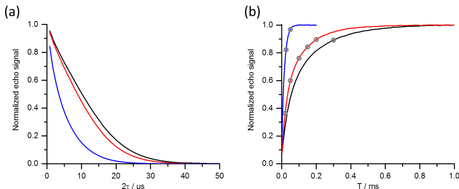
Figure 3. Echo decay traces (a) and SR traces (b) of the Gd(III)-DOTA ruler at 5 K (black), 10 K (red), and 25 K (blue). Circles on the SR traces mark the T_{mix} values used for RIDME experiments. The magnetic field was set to the maximum of the EPR spectrum for both experiments. (The curves presented in a logarithmic scale are shown in Fig. S1)
