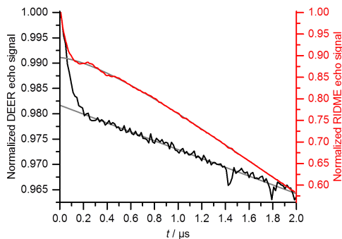
Figure 6. Comparison of background decays in DEER and RIDME experiments for the Gd(III)-DOTA ruler. Normalized primary dipolar evolution traces of the DEER (black) and RIDME (red) traces of Figs. 4 and 5, respectively, are shown together with the background fits (grey lines).
