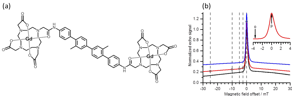
Figure 2. Molecular structure of the Gd(III)-DOTA ruler (a) and W-band ED-EPR spectra (b). The spectra were recorded at 5 K (black), 10 K (red), and 25 K (blue). The inset shows a
