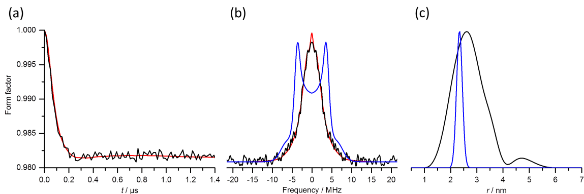
Figure 4. DEER measurements of the Gd(III)-DOTA ruler. (a) DEER form factor (black line) and fit (red line) obtained at T = 10 K with \Delta\nu = 100 MHz. (b) Comparison between the Fourier transforms of the experimental (black) and fitted (red) DEER form factor and the expected Pake pattern for a S = \frac{1}{2} spin system characterized by an inter-spin distance of 2.35 nm with a distance distribution width of 0.25 nm (blue). (c) Distance distribution obtained from Tikhonov regularization of the DEER form factor ( \alpha = 1000 ; black) and expected distance distribution (blue).
