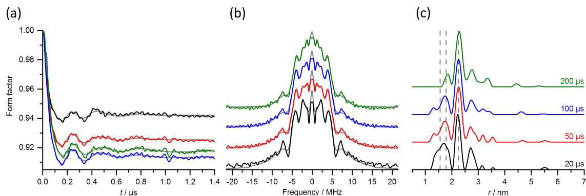
Figure 7. 10 K RIDME measurements of the Gd(III)-DOTA ruler with different T_{\text{mix}} values as indicated on the figure. (a) Form factors with corresponding fits (grey). (b) Corresponding Fourier transforms of the experimental data (colored) and fits (grey). (c) Distance distributions obtained by Tikhonov regularization of the RIDME form factors ( \alpha = 1 ). The grey dashed lines denote, from right to left, the mean distances corresponding to the first, second and third harmonic of the electron-electron dipolar interaction. The color codes are the same for all panels.
