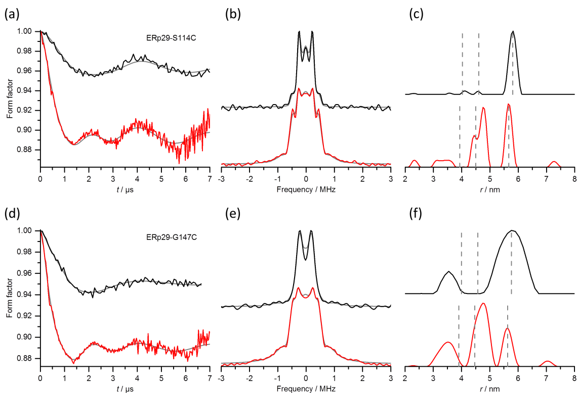
Figure 10. (a) – (c) RIDME and DEER experiments of ERp29 S114C-C9-Gd(III). (a) RIDME (red) and DEER (black) form factors and fits (grey) for experiments performed at T = 10 K, using \Delta\nu = 100 MHz in the DEER experiment and T_{\text{mix}} = 25 \mu\text{s} in the RIDME experiment. (b) Fourier transforms of the RIDME and DEER form factors (red and black, respectively) and fits (grey). (c) Distance distributions obtained from Tikhonov regularization of the RIDME and DEER form factors ( \alpha = 10 ). The grey dashed lines denote, from right to left, the mean distances corresponding to the first, second, and third harmonics of the electron-electron dipolar interaction. (d) – (f) RIDME and DEER experiments of ERp29 S147C-C9-Gd(III). The same measurement conditions and data analysis protocol were used as in (a) – (c).
