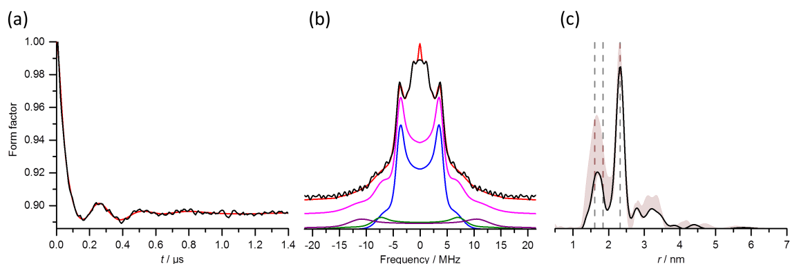
Figure 5. RIDME measurements of the Gd(III)-DOTA ruler. (a) RIDME form factor (black) and fit (red) obtained at T = 10 K with T_{\text{mix}} = 150 \mu\text{s} . The ripple on the experimental trace arises from ^2\text{H} modulations ( \nu_1 \approx 22.5 MHz; see Fig. S3b). (b) Fourier transforms of the RIDME form factor (black) and fit (red). The magenta line shows the expected overall frequency
