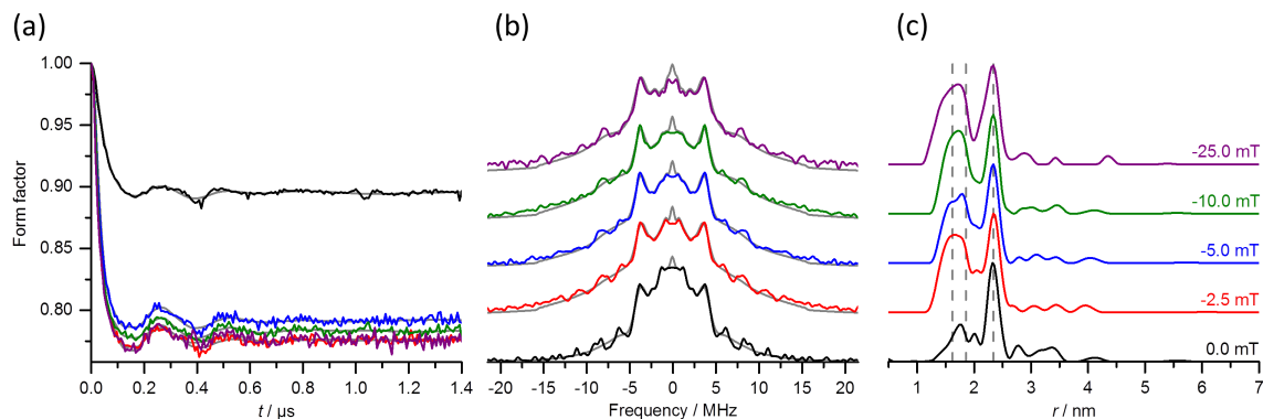
Figure 8. RIDME measurements of the Gd(III)-DOTA ruler as a function of the magnetic field position within the EPR spectrum. (a) Form factors measured at \Delta B_0 indicated on the figure, where \Delta B_0 is the field offset with respect to the maximum of the EPR spectrum, with corresponding fits (grey). Measurements were performed at T = 10 \text{ K} with T_{\text{mix}} = 150 \mu\text{s} . (b) Fourier transforms of the form factors and fits shown in (a). (c) Distance distributions obtained from Tikhonov regularization of the RIDME form factors ( \alpha = 1 ) in (a). The grey dashed lines denote, from right to left, the mean distances corresponding to the first, second, and third harmonic of the electron-electron dipolar interaction. Same color codes are used for all three panels.
