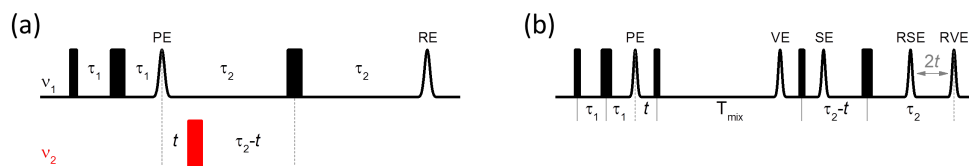
Figure 1 Pulse sequences of the 4-pulse DEER 23 (a) and 5-pulse RIDME 24 (b) experiments. In the 4-pulse DEER experiment the intensity of the refocused echo (RE) is modulated by the electron-electron dipolar interaction as a function of the time t , which defines the position of the \pi pulse at the second MW frequency \nu_2 . PE is the primary echo. In the 5-pulse RIDME experiment the intensity of the refocused virtual echo (RVE) is modulated by the electron-electron dipolar interaction as a function of the time t , which defines the position of the third and fourth pulses. VE, SE and RSE are the virtual, stimulated and refocused stimulated echoes, respectively.
