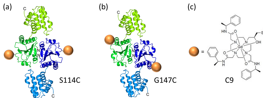
Figure 9. Structures of the ERp29 homodimer with C9-Gd(III) tag. 15 (a) Ribbon representation of the S114C mutant. (b) G147C mutant. (c) Molecular structure of the C9-Gd(III) tag.
