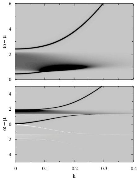
FIG. 2. Absorption coefficient vs momentum ( x axis) and energy ( y axis) calculated above (top) and below (bottom) phase transition. Negative values indicate gain. (Parameters as for Fig. 1, inhomogeneous broadening width 0.3g\sqrt{n} .) The color scale covers the range -\infty to \infty .
