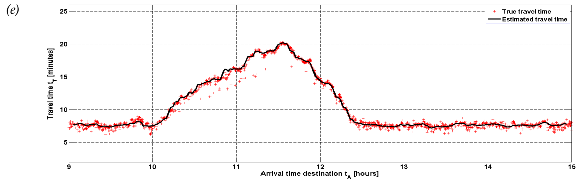
Figure 2. A graphical representation of the score matrix at some important steps within the travel time estimation procedure: (a) Raw score matrix (b) Score matrix after convolution, (c) Score matrix after weighting of the diagonals, (d) Score matrix after resizing and filtering, (e) Estimated travel time after finding the path with maximum costs from (2d), and comparison of estimated travel times (black line) with true travel times (red crosses).
