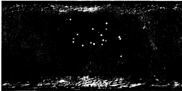
Figure 1. LROC WAC mosaic showing the locations of the 22 young, fresh mare craters studied here. Squares show craters with visible layering structures in the craters walls as identified by Sharpton (2014) [3]. Colors represent general categories of profile shape.
