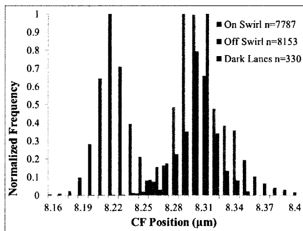
Figure 1. CF position distributions measured on the Reiner Gamma Swirl (blue), in typical off-swirl terrain (green), and within the anomalously low albedo dark lane (red).
