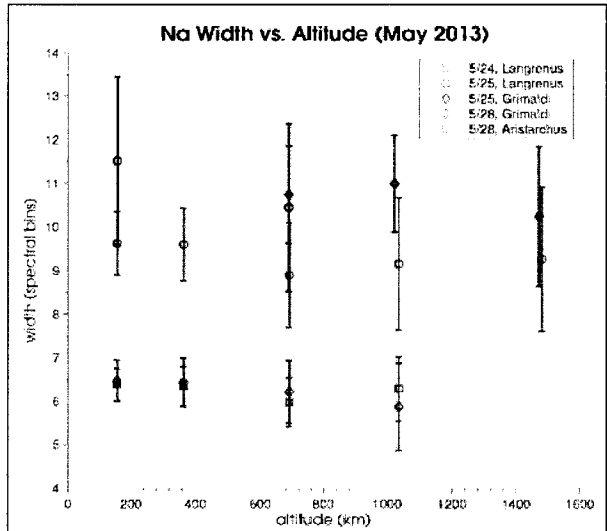
Figure 3. The Na widths (FWHM) are plotted vs the distance to the center of a 3' FOV (312 km). The FOV was moved from the limb due East of the Langrenus crater (61.1° E, 8.9°) and due West of the Grimaldi crater (68.3° W, 5.5° S) and the Aristarchus crater (47.4° W, 23.7° N). The full moon was May 25 at a distance of 356,000 km. The lunar phase angles were 13°, 2° and 44° for May 24, 25 and 28, respectively.
