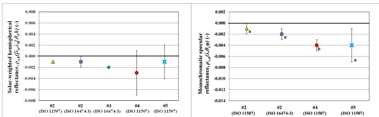
FIGURE 9. Average of the solar-weighted hemispherical reflectance differences (left) and monochromatic specular reflectance differences (right) after UV light and humidity test.
