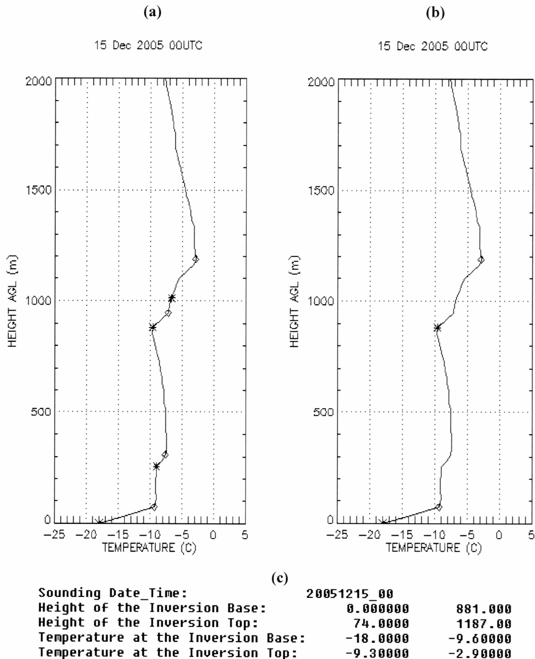
Figure 2.6 Inversion layers detected by the algorithm. (a) Temperature profile showing the four inversion layers initially detected by the algorithm. The * represents the base and the \diamond represents the top of the of the inversion layers (b) Final two inversion layers selected by algorithm (c) Altitude and temperature data for the two inversion layers shown in Fig. 2.6b.
