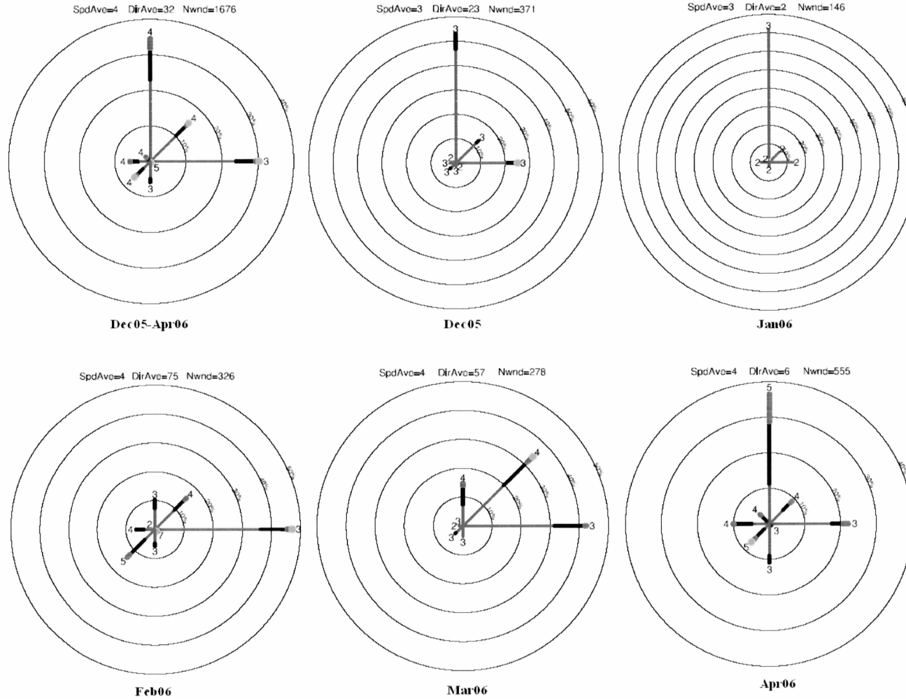
Figure 3.11 Wind roses from sodar. Wind roses from sodar observations taken at one hour intervals at an average altitude of 70m AGL.
