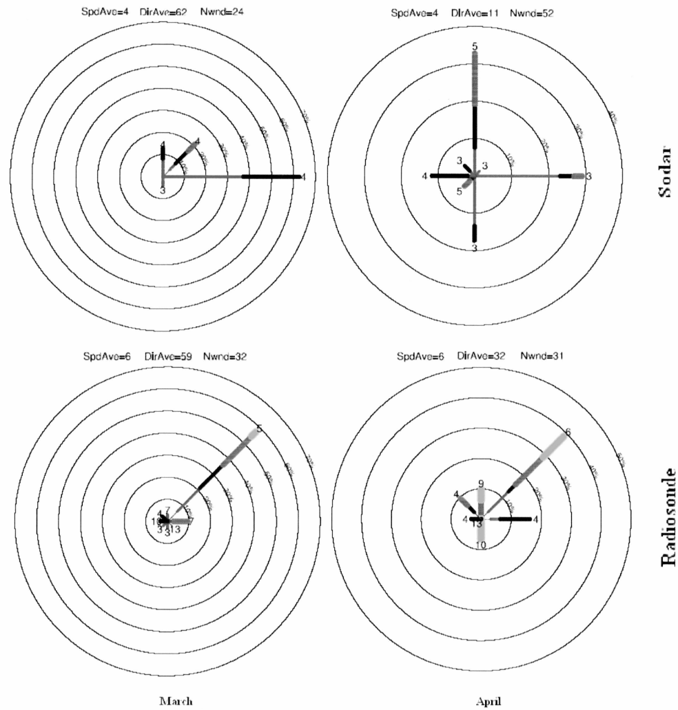
Figure 3.10 (b) Wind roses explained in Fig. 3.10 (a) for the months of March and April
