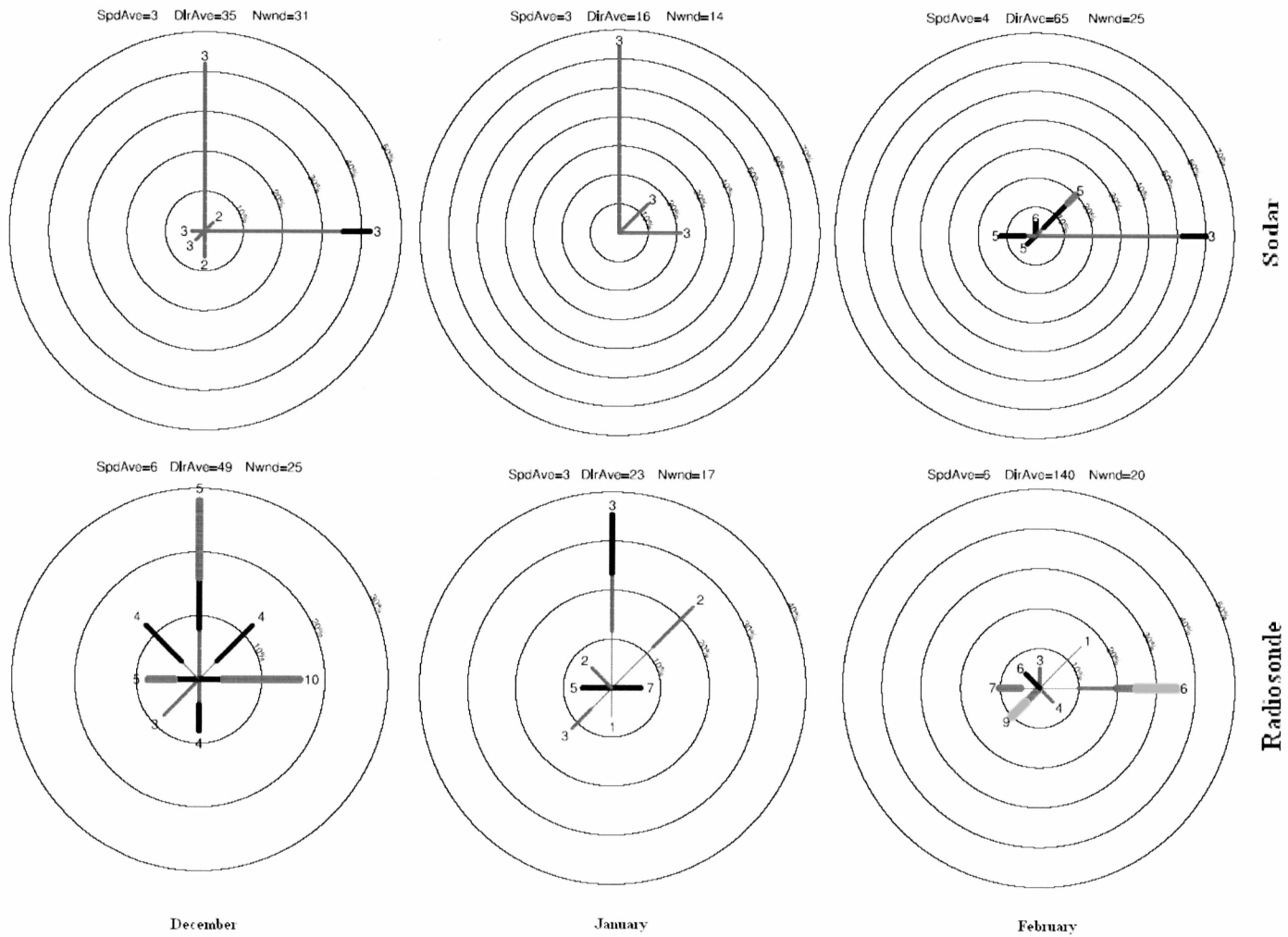
Figure 3.10a Wind roses - month wise. (a) Wind roses plotted separately for the months of December, January and February using the same data as in Fig. 3.9.
