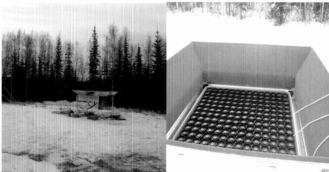
Figure 2.2 Doppler sodar at the NWS site in Fairbanks. (Left) Doppler sodar antenna installed at the NWS site in Fairbanks. (Right) Closer look at the phased array antenna. It comprises of 196 transducers mounted on four panels and surrounded by sound absorbing cuffs to suppress side lobes and to reduce unwanted background noise. The three white heating cables seen on the right are passed along the base of the antenna elements to thaw the snow accumulated from precipitation. (Photos by the author).
