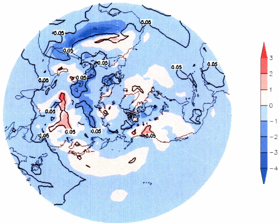
Figure 3.13 JJA surface air temperature composite anomalies ( ^{\circ}\text{C} ) for years with extreme low area burned. Areas of significant p=0.05 anomalies contoured.
