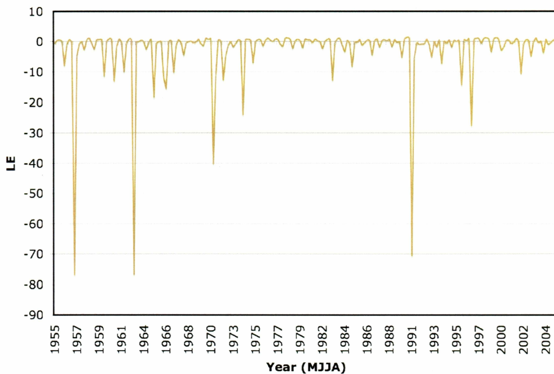
Figure B.1 May, June, July, and August dryness index for the Lettau Climatology (LE) calculated from Equation B.1.
