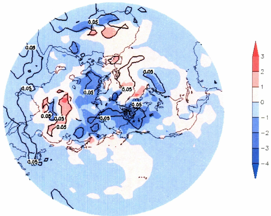
Figure 3.11 MAM surface air temperature composite anomalies ( ^{\circ}\text{C} ) for years with extreme low area burned. Areas of significant p=0.05 anomalies contoured.
