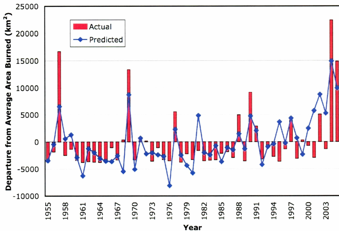
Figure 3.18 Results of the preseason multiple regression plotted as departure from average area burned. Blue line is the results of the multiple regression and solid red columns are the observed area burned.
