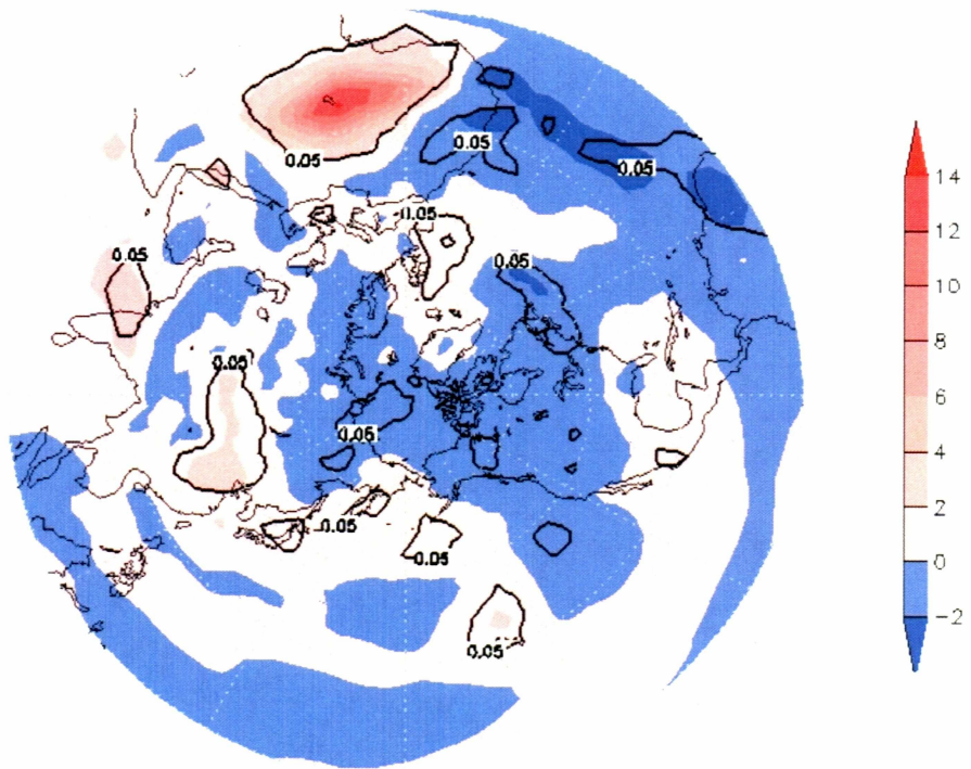
Figure 3.9 MAM total column precipitable water composite anomalies ( \text{kg/m}^2 ) for years with extreme low area burned. Areas of significant p=0.05 anomalies contoured.
