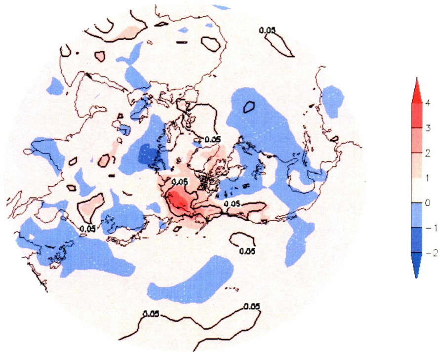
Figure 3.5 MAM surface air temperature composite anomalies ( ^{\circ}\text{C} ) for years with extreme high area burned. Areas of significant p=0.05 anomalies contoured.
