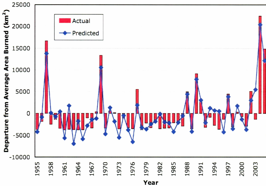
Figure 3.16 Results of the spring and summer multiple regression plotted as departure from average area burned. Blue line is the results of the multiple regression and solid red columns are the observed area burned.
