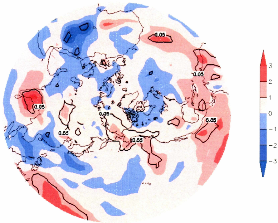
Figure 3.4 MAM total column precipitable water composite anomalies ( \text{kg}/\text{m}^2 ) for years with extreme high area burned. Areas of significant p=0.05 anomalies contoured.
