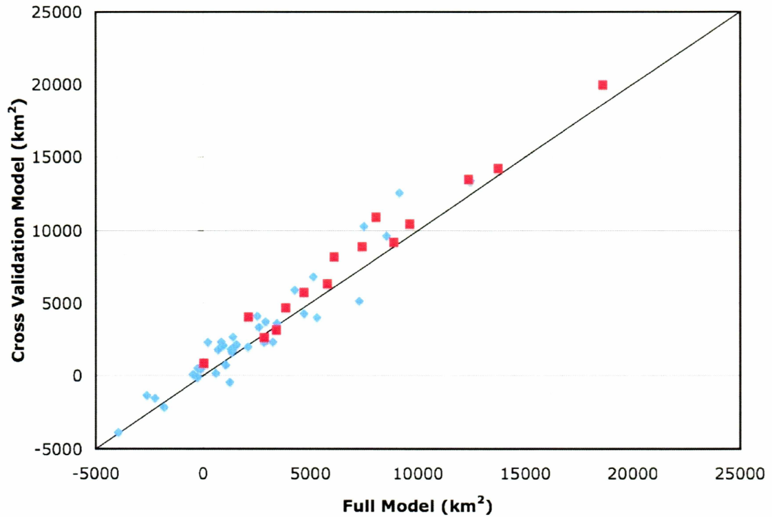
Figure 3.19 Full model versus the model fitted 1955-1990 (blue diamonds) and 1991-2005 (red squares) predicted for the preseason multiple regression.
