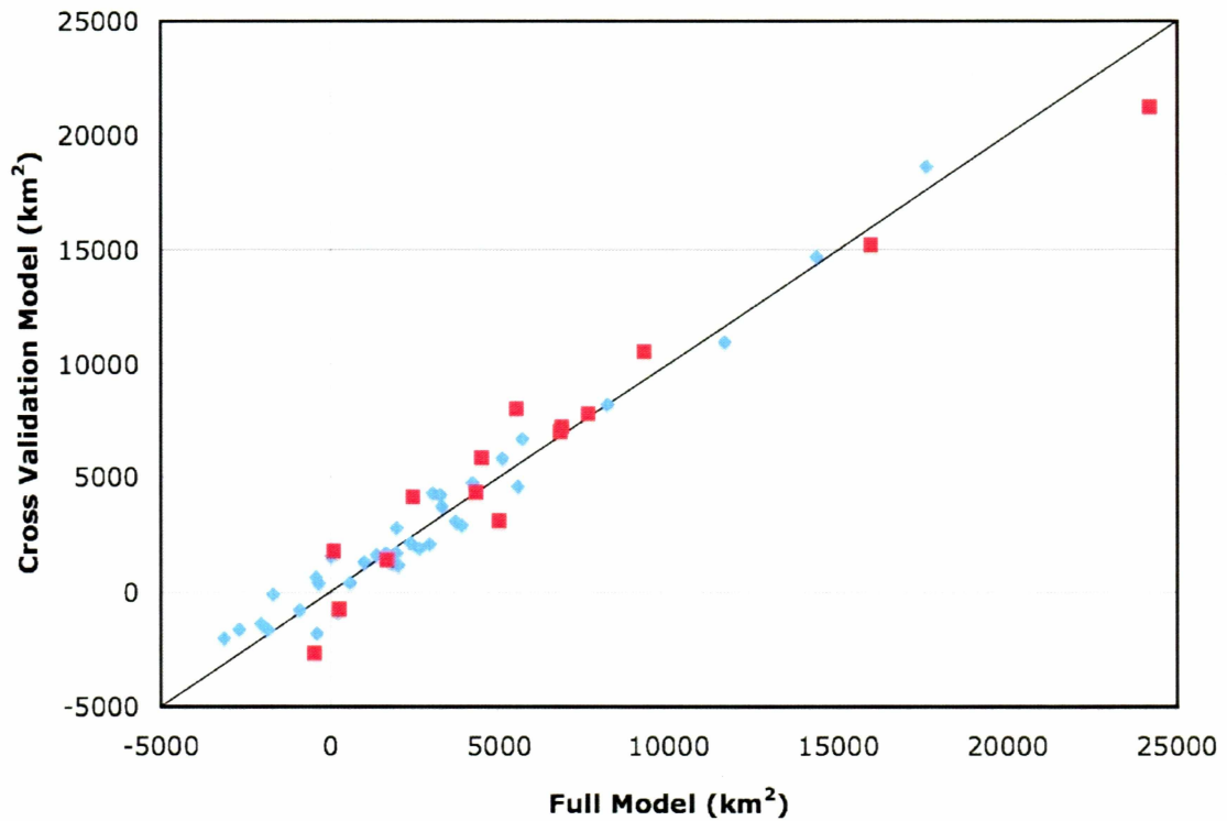
Figure 3.17 Full model versus the model fitted 1955-1990 (blue diamonds) and predicted 1991-2005 (red squares) for the spring and summer multiple regression.
