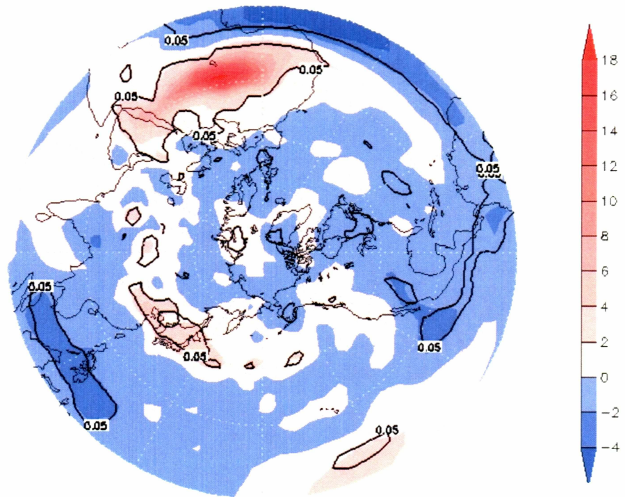
Figure 3.12 JJA total column precipitable water composite anomalies ( \text{kg/m}^2 ) for years with extreme low area burned. Areas of significant p=0.05 anomalies contoured.
