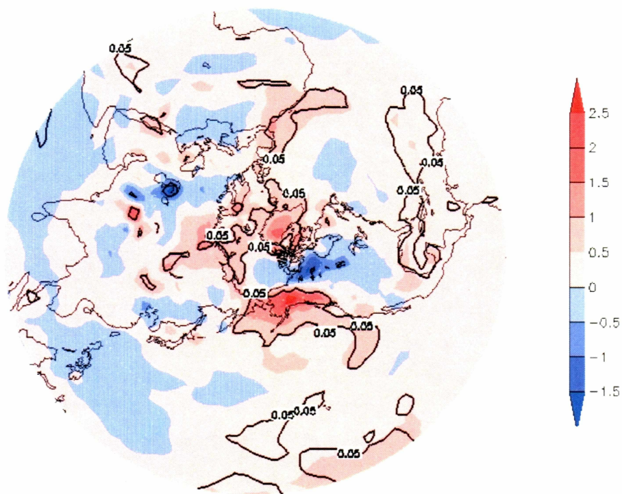
Figure 3.8 JJA surface air temperature composite anomalies ( ^{\circ}\text{C} ) for years with extreme high area burned. Areas of significant p=0.05 anomalies contoured.
