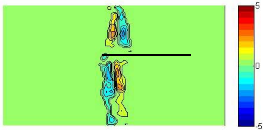
Figure 4.27: Water Aluminum 5 V 15 Hz Vorticity Plot
