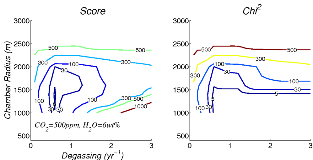
Figure 3.8: The results from the fixed volatile content models are summarized in the contour plot. The \chi^2 and total score values are contoured for models with volatile concentrations of 500ppm \text{CO}_2 and 6wt.% \text{H}_2\text{O} . Together the two contour plots are useful in assessing how well the models fit the data. The \chi^2 plot (right) shows that for magma with this volatile content, magma chambers must be less than \sim 2\text{km} in radius, and that a degassing rate greater than \sim 0.5\text{yr}^{-1} is adequate to fit the data. The overall score (left) indicates that the high degassing rates result in exorbitant \text{CO}_2 fluxes. The result is that chamber sizes in the range \sim 1\text{-}2\text{km} and degassing rates between 0.5 and 1\text{yr}^{-1} best fit the data. Both \chi^2 and score values are unitless. Models with \chi^2 or score less than \sim 30 or less are acceptable models.
