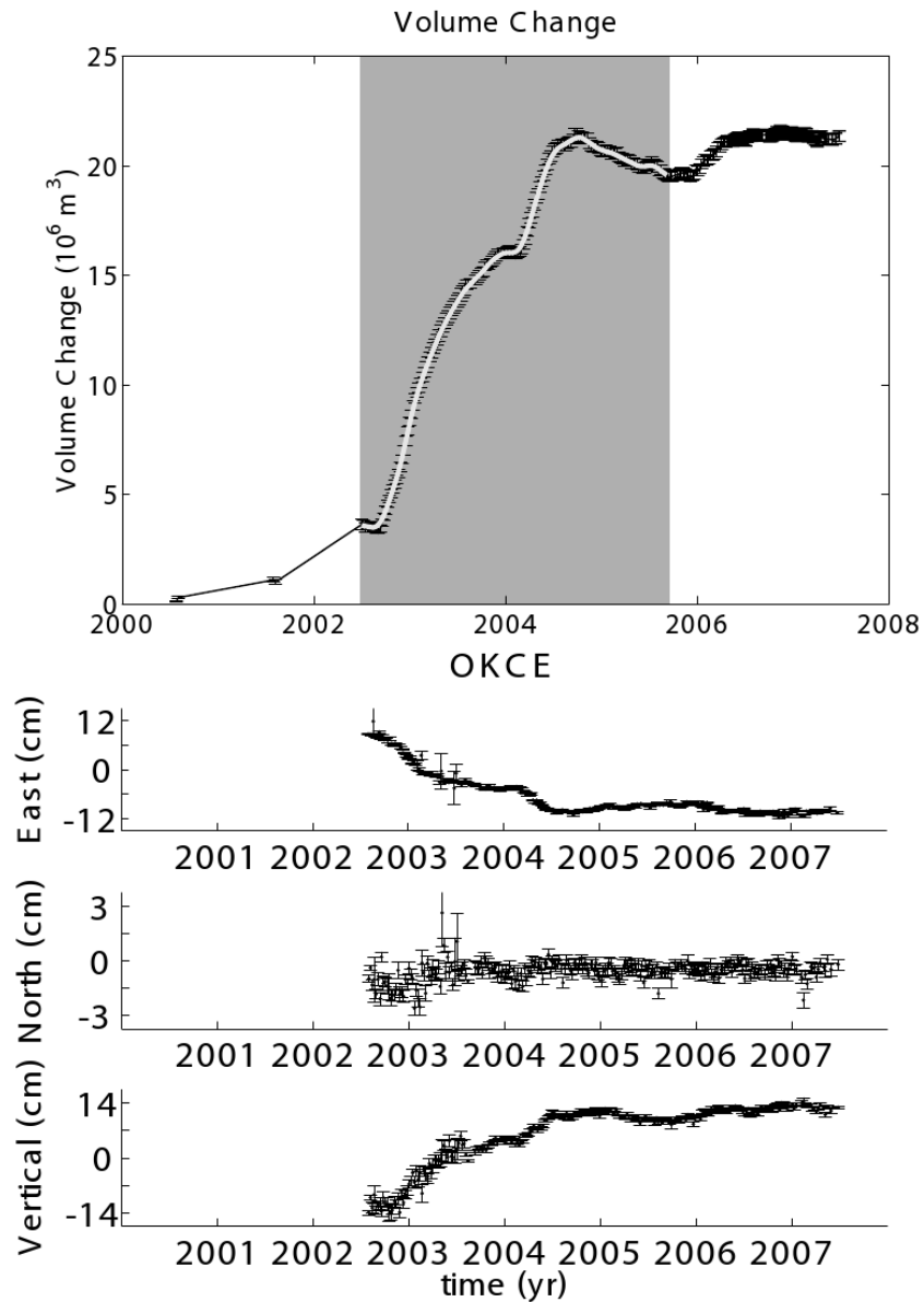
Figure 3.2: The volume change of the magma chamber beneath Okmok is tracked through time with the GPS network [Fournier et al. , 2008; Chp. 2 ]. The top panel shows the estimate of the cumulative volume change since 2000, the period of time that this study focuses on is shown in gray. The white line is the smoothed volume change curve used as data in the study. The bottom panel shows the three component site motion of OKCE.
