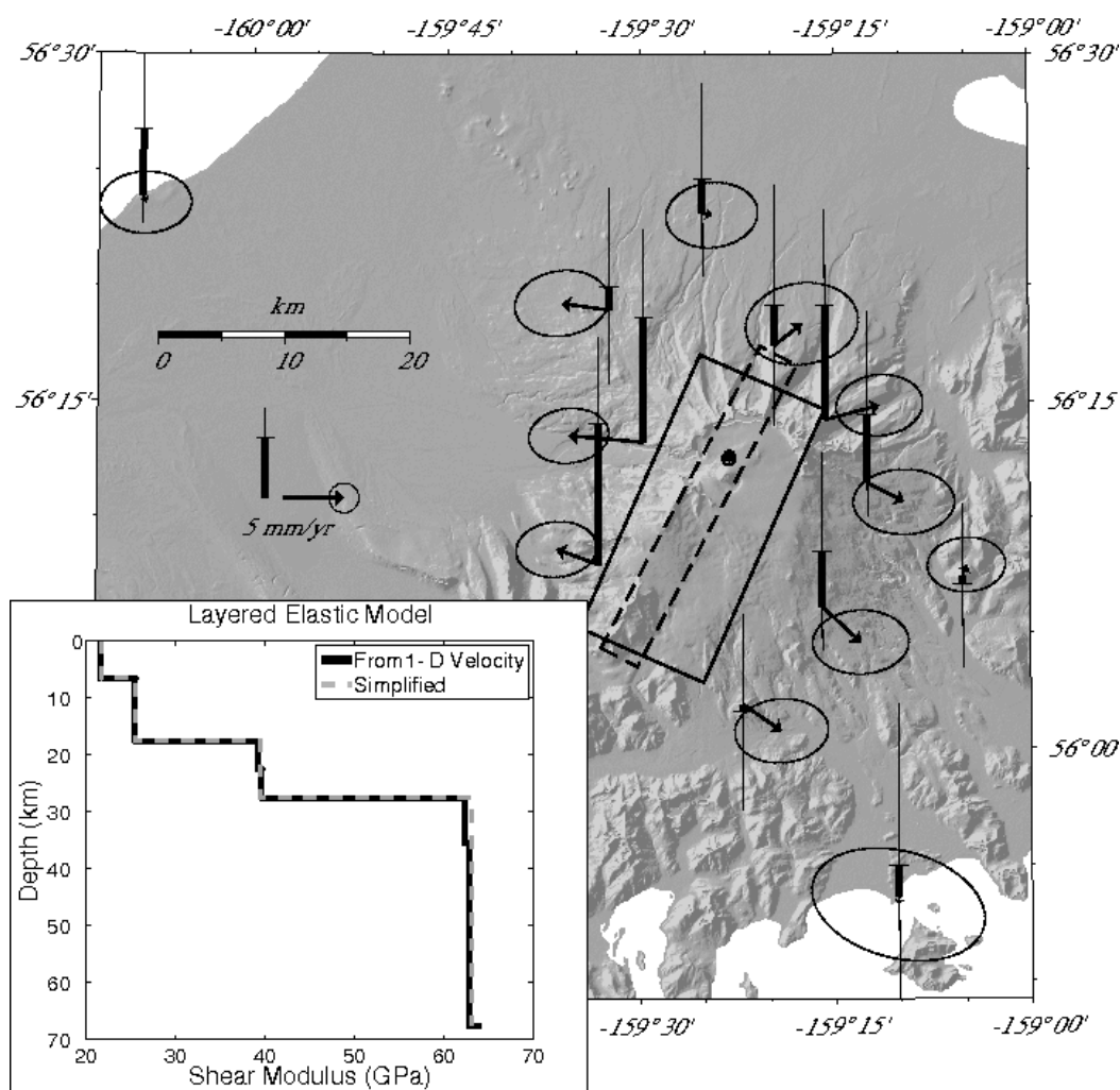
Figure 5.2: The GPS velocities highlight the volcano deformation after the tectonic component has been removed from the observed North America relative velocities (Figure 5.1). Horizontal velocities are indicated by the arrows with 95% confidence ellipses. Vertical velocities are the vertical bars with a horizontal bar indicating up or down motion. The 95% confidence interval for the vertical component is indicated by the thin vertical line. The best fitting models are shown; sill in homogeneous half-space (solid line), sill in a layered half-space (dashed line), Mogi source in a homogeneous half-space (solid dot), Mogi source in a layered half-space (open dot) (note that the both Mogi sources are in almost the exact same location). The layered model, calculated using a p-wave velocity model [Sanchez, 2005] is shown in the inset (black). The elastic structure is simplified into a four layer model (grey dashed) that is used for the deformation source inversions.
