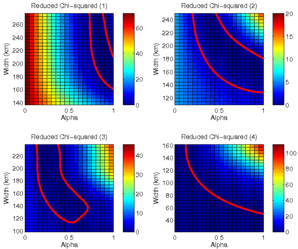
Figure 4.5: Misfit plots of width vs. slip-deficit for each plane in the modeled subduction interface. The figure shows the reduced-chi-squared values for models with varying width and parameter alpha. Alpha is a parameterization of slip-deficit where alpha multiplied by the convergence velocity is equal to the slip deficit. The red line in each panel is the 95% confidence contour. Panels 1-4 correspond to the model planes 1-4 described in the text.
