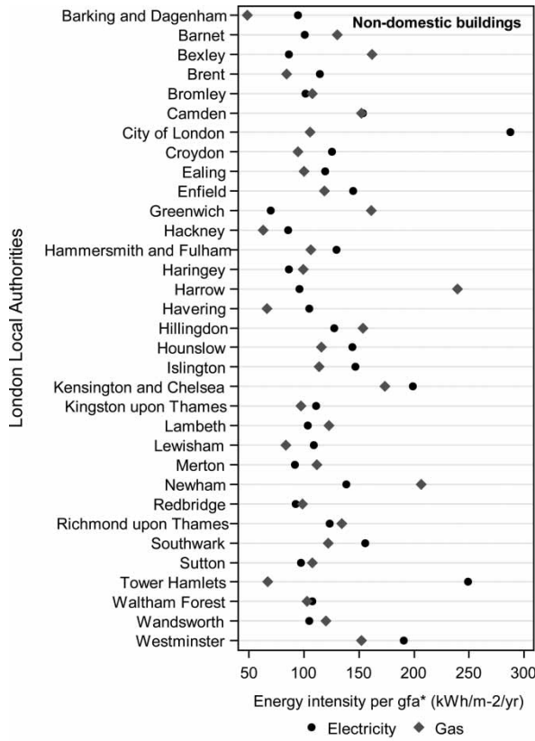
Figure 7 Non-domestic electricity and gas intensity per m 2 of gross floor area for London's local authorities
