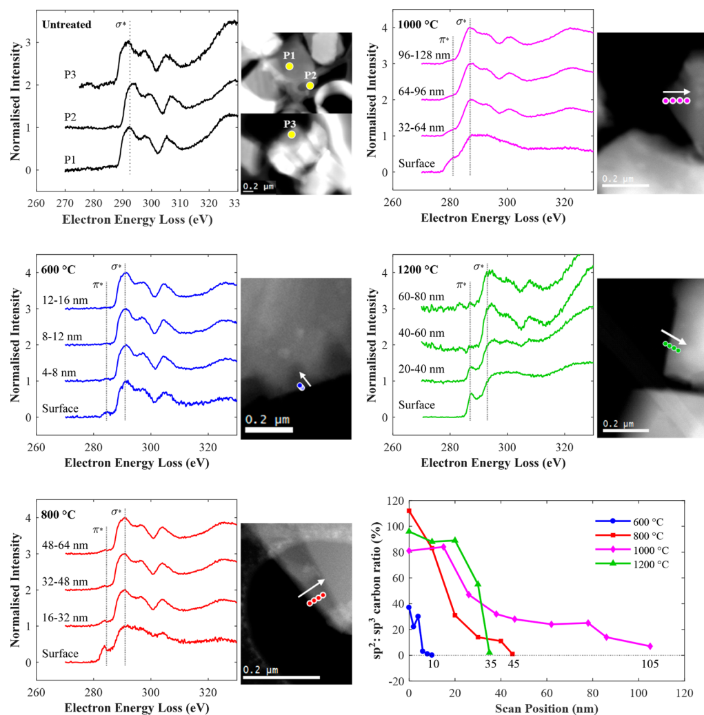
Figure 4. STEM–EELS of the annealed diamond powders at different locations on a particle. The arrow denotes the direction from the surface inward into the particle. No evidence of any sp^2 carbon was found at various points on the initial untreated samples. The annealed samples showed sp^2 carbon layers with approximate thicknesses of 10, 45, 105, and 35 nm for 600, 800, 1000, and 1200 °C, respectively.
