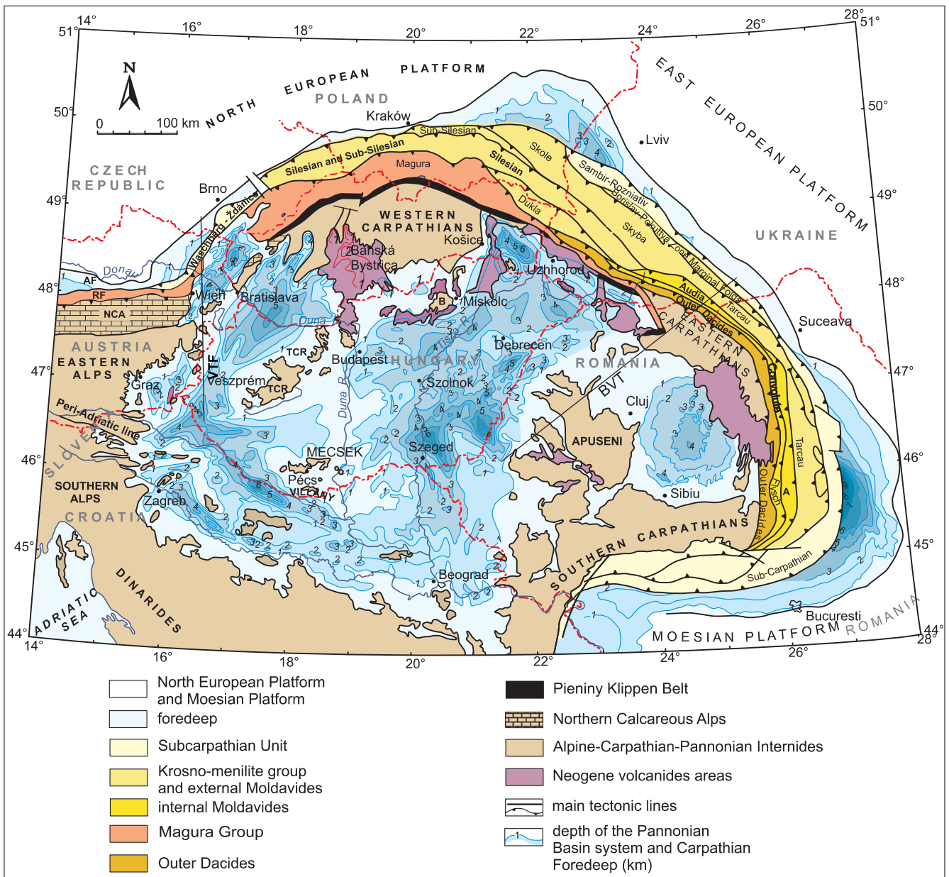
Fig. 1. Geological map of the East Alpine–Carpathian–Pannonian basin system (after Kovač et al. , 1998)
