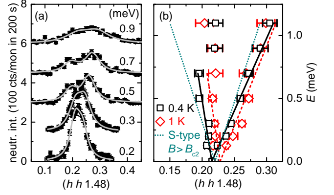
FIG. 2. Dispersion of the magnetic mode in A-type \text{CeCu}_2\text{Si}_2 . (a) Scans along [110] at 0.4 K for several energy transfers, as well as Lorentzian fit functions (solid lines). Data are displayed after background subtraction and with an offset of 150 counts. (b) Fitted peak positions of the magnetic mode for 0.4 K and 1 K. Linear fits for the dispersion relation are shown in solid or dashed lines, respectively (details see main text). The dotted line shows the dispersion of S-type \text{CeCu}_2\text{Si}_2 in the normal state ( B = 1.7 T, T = 60 mK) 23 .
