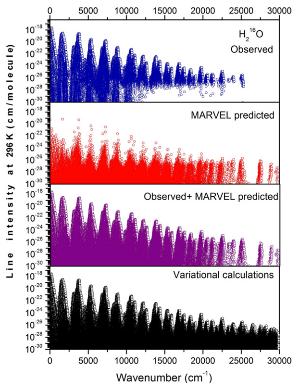
Fig. 3. Comparison of intensities at 296 K for one-photon absorption transitions of \text{H}_2^{16}\text{O} up to 30\,000\text{ cm}^{-1} . Top panel—measured lines; second panel—MARVEL predicted but omitting the above observed line; third panel—sum of the first two; and bottom panel—all lines predicted by variational computations (BT2 [194]). The weakest measured intensities come from emission spectra of hot water which are difficult to obtain directly in absorption.
