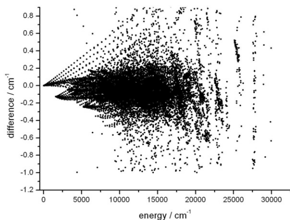
Fig. 2. Differences between the present MARVEL energy levels and their counterparts present in the BT2 linelist [194].
