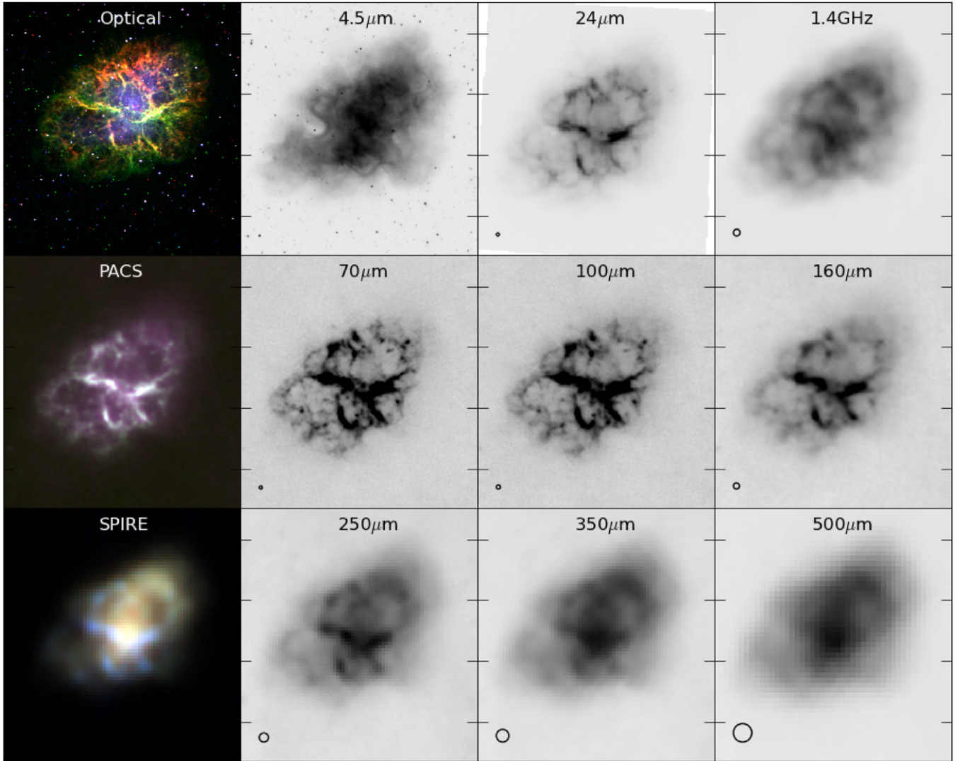
Figure 2. Multiwavelength montage of the Crab SNR centered on the pulsar (R.A. = 262:671, decl. = 22:0145, J2000.0) with diameter 4'2 \times 4'2 . Top (from left to right): three-color image in H \alpha (red), [O III] (green), and Bessel B (blue) using images obtained from the Faulkes Telescope North (Appendix A). Spitzer IRAC 4.5 \mu\text{m} , MIPS 24 \mu\text{m} , and VLA archive data at 1.4 GHz (taken in 1996). Middle: Herschel PACS three-color image and individually the 70, 100, and 160 \mu\text{m} images. Bottom: Herschel SPIRE three color image and individually, 250, 350, and 500 \mu\text{m} images. Beam sizes are indicated with the black circle in the lower left corner. (A color version of this figure is available in the online journal.)
