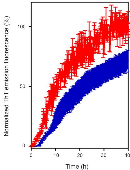
Fig. S2. Effect of seeding on the mechano-enzymatic mechanism of TTR amyloid fibrillogenesis. Normalized ThT fluorescence emission of S52P TTR at 1 mg/ml in the presence (red) or in the absence of seeds (blue) during incubation with 20 ng/ \mu l of plasmin. ThT emission fluorescence of the TTR plasmin-related seeds (0.1 mg/ml) added to the reaction was subtracted before normalization. Data plotted as mean \pm s.d. of three replicates.
