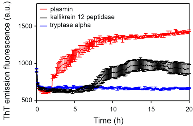
Fig. S1. Effect of tryptase alpha and kallikrein 12 on S52P TTR. Amyloid fibrillogenesis of S52P TTR in the presence of tryptase alpha, kallikrein 12 peptidase and plasmin in a 1:50 enzyme/substrate ratio monitored in the presence of fluid agitation and 10 \mu M ThT at 37°C. Means \pm s.d. of three replicates are shown.
