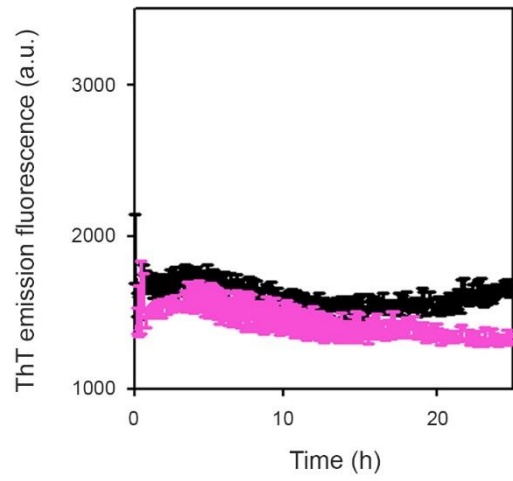
Fig. S3. Effect of plasmin on TTR amyloid fibrils. Relative intensities of ThT fluorescence of S52P TTR fibrils at 0.1 mg/ml in the presence (black) and in the absence (magenta) of plasmin at an enzyme:substrate ratio of 1:50. Data plotted as mean \pm s.d. of three replicates.
