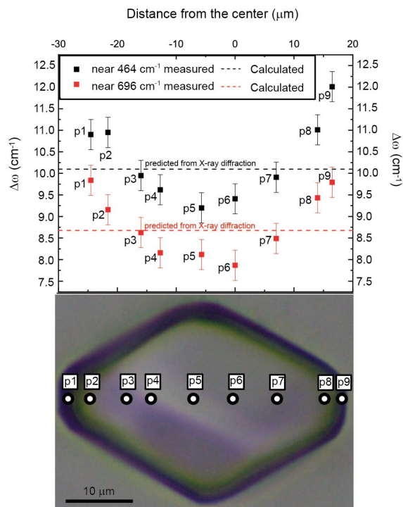
FIGURE 4. Wavenumber shifts of the 464 and 696 \text{cm}^{-1} modes measured in a traverse across a quartz inclusion in pyrope from the eclogite xenolith TM90-1 (Korsakov et al. 2009). The phonon wavenumber shifts calculated from the strains determined by X-ray diffraction and the mode Grüneisen tensor are in good agreement with the average of the measured shifts.
