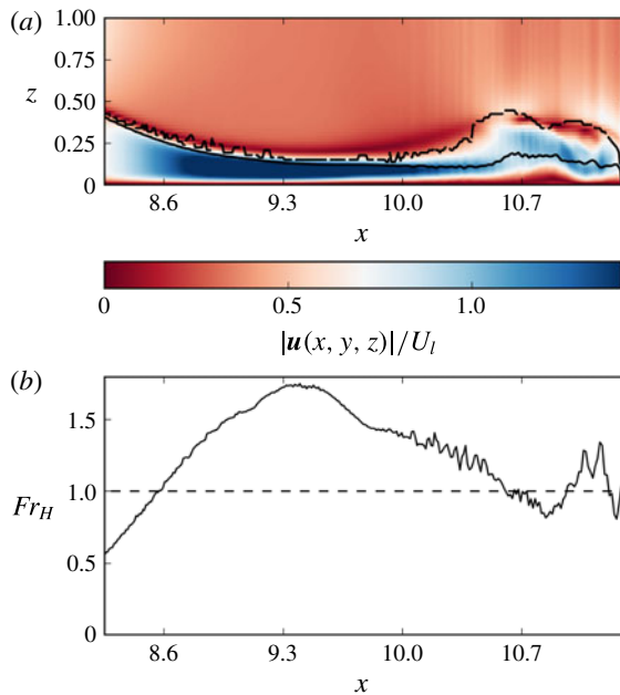
FIGURE 8. (a) Non-dimensional velocity |u|/U_l on the mid-plane y = y_0 ; the thick black line indicates the depth h_l = \overline{g'h/g'} and the dashed line marks h_t , i.e. the interface \rho = 3\% , (b) Froude number Fr_H versus x . Case S3, t = 8.7 .
