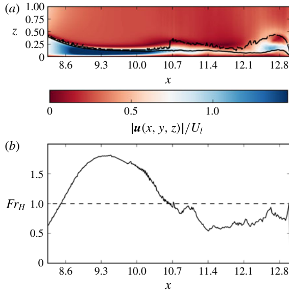
FIGURE 9. (a) Non-dimensional velocity |u|/U_l on the mid-plane y = y_0 ; the thick black line indicates the depth h_l = \overline{g'h}/g' and the dashed line marks h_i , i.e. the interface \rho = 3\% , (b) Froude number Fr_H versus x . Case S3, t = 16 .
