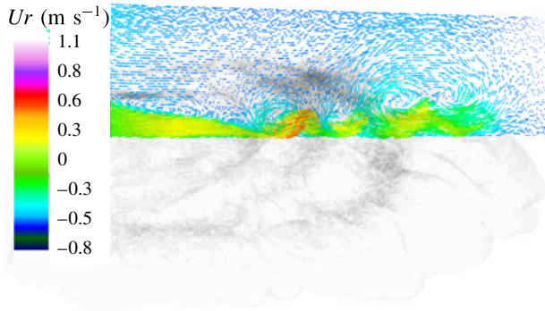
FIGURE 15. Case S11: velocity field on the mid-plane (x, y) , Gr = 8.1 \times 10^8 , \epsilon = 0.03 , t = 12 .
