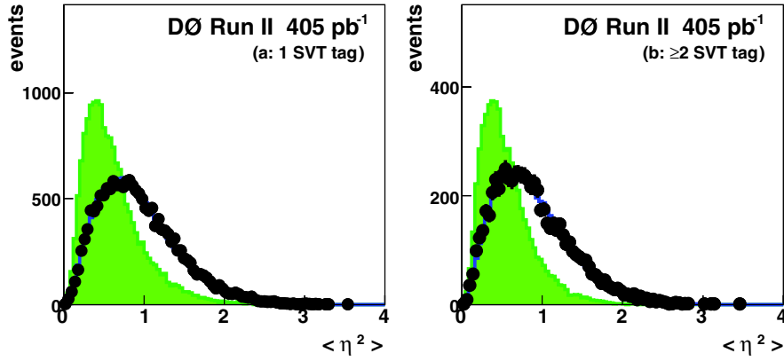
FIG. 4 (color online). The \langle \eta^2 \rangle distribution for single-tag events (a) and double-tag events (b). Shown are the data (points), the background (solid line), and the expected t\bar{t} distribution (filled histogram) multiplied by 140 (60) for the single (double)-tag analysis.
