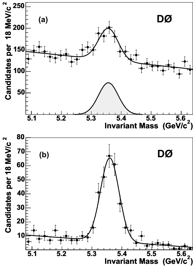
FIG. 1. (a) Mass distribution for B_s^0 candidate events. Points with error bars show the data, and the solid curve represents the result of the fit. The mass distribution for the signal is shown in gray; (b) same distribution after requiring the significance of the lifetime measurement to be c\tau/\sigma(c\tau) > 5 .
