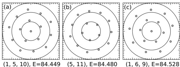
Figure 1. Ground (a) and metastable (b, c) states of a 16-particle 2D Coulomb cluster. The concentric circles mark equipotential lines of the parabolic trap. Numbers in parentheses list the numbers of particles in each shell starting with the innermost one. Note that the energy differences are quite small.
