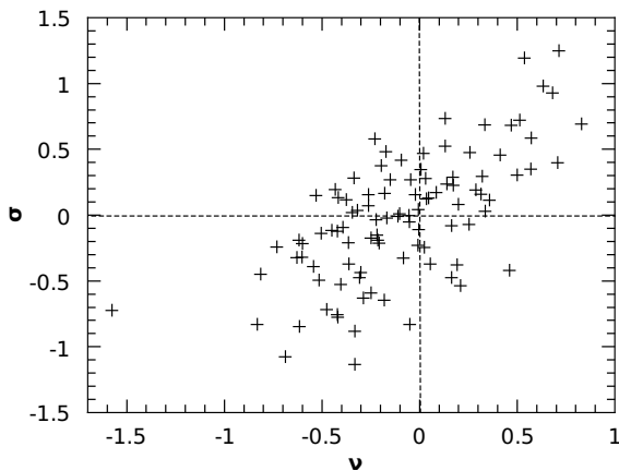
Figure 9. Correlations between fluctuations of entropy \sigma and the logarithm of the number of discovered stable configurations \nu in a 2D system with screening constant \kappa = 1 .
