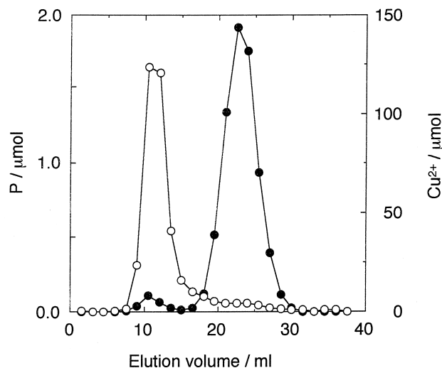
Fig. 4 Elution profiles of the Cu 2+ -EDTA complex and MLVs containing Cu 2+ by gel-filtration. Conditions: column, Sephadex G-50 (10 × 300 mm); mobile phase, 10 mM Mops buffer (pH 7.5); MLVs suspensions, 275 μl; flow rate, 0.3 ml/min; fractionation, 5 min/tube. (○), phosphorus; (●), copper.
