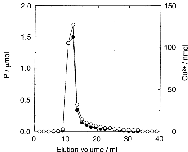
Fig. 1 Elution profiles of MLVs containing \text{Cu}^{2+} obtained by gel-filtration. Conditions: column, Sephadex G-50 (10 × 300 mm); mobile phase, 10 mM Mops buffer (pH 7.5); MLVs suspensions, 275 \mu l; flow rate, 0.3 ml/min; fractionation, 5 min/tube. (○), phosphorus; (●), copper.
