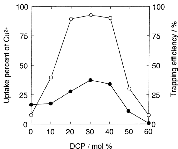
Fig. 3 Effect of the molar composition of DCP in MLVs on the uptake percent of Cu 2+ and the trapping efficiency of calcein. Conditions: total mol of PC, Chol and DCP was kept constant at 42 μmol and the mol% of Chol was kept constant at 30 mol%. (○) uptake of Cu 2+ ; (●) trapping efficiency of calcein.
