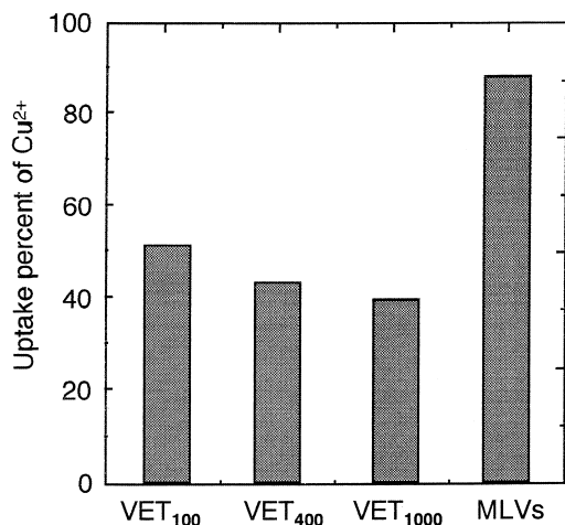
Fig. 2 Effect of the liposome size on the uptake percent of Cu 2+ . Conditions: liposome suspensions, 0.9 ml; solution of Cu 2+ , 0.1 ml; mixing time, 30 min.
