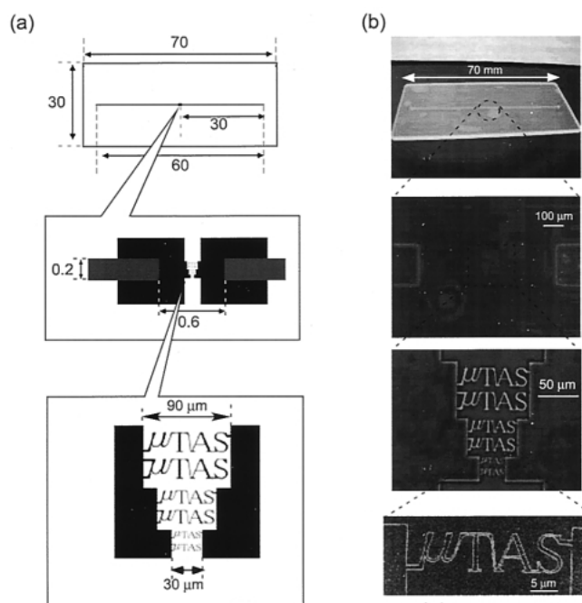
Fig. 2 (a) Layout of the complicated nano channels. The depths of the gray pattern and black pattern were 50\ \mu\text{m} and 250\ \text{nm} , respectively. (b) The top picture is a photograph of the chip. The middle two pictures are optical micrographs and the bottom picture is an SEM image of the complicated nanochannels connected to the microchannels for liquid introduction.
