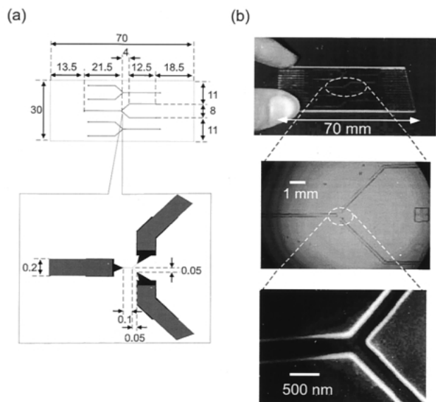
Fig. 1 (a) Layout of the nano chemical reactor. The depths of the gray pattern and black pattern were 40\ \mu\text{m} and 400\ \text{nm} , respectively. The numbers in this figure are “mm”. (b) The top two pictures are optical micrographs of the nano chemical reactor, and the bottom picture is an electron micrograph of it.
