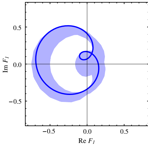
FIG. 3. F_1 in the model 1.
