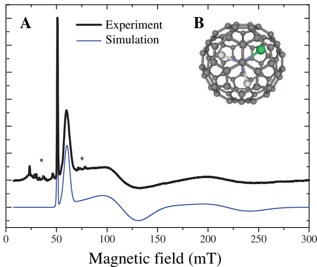
FIG. 1 (color online). (a) X-band cw EPR spectrum of \text{ErSc}_2\text{N@C}_{80} in frozen toluene solution at 5 K, with accompanying simulation performed using EASYSIPIN [23]. The low-intensity sharp features marked * derive mostly from hyperfine coupling to the ^{167}\text{Er} nuclear spin (natural abundance 22.9%). Experimental parameters: microwave frequency, 9.396 GHz; microwave power, 63 mW; modulation amplitude, 0.3 mT; modulation frequency, 100 kHz. (b) A representation of the \text{ErSc}_2\text{N@C}_{80} molecule.
