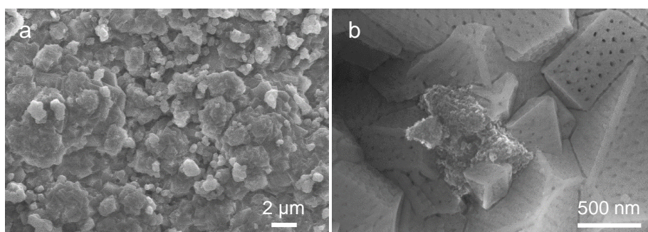
Figure 4. SEM images of the surface of the Al-TiO 2 composite coating containing 8 vol% TiO 2 after anodization.
