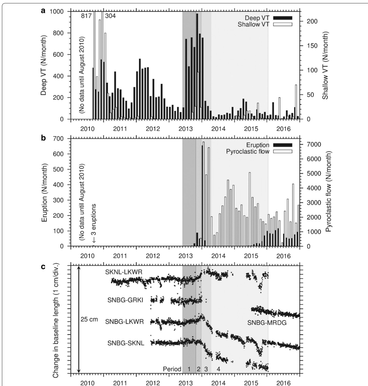
Fig. 2 a Monthly numbers of deep (black) and shallow (white) VT earthquakes at Sinabung occurring between September 2010 and December 2016. b Monthly number of eruptions (black) and pyroclastic flows (white) at Sinabung occurring between September 2010 and December 2016. c Examples of the temporal change in baseline lengths. Periods 1–4 are analysis periods defined based on the characteristics of ground deformation (Hotta et al. 2017)
