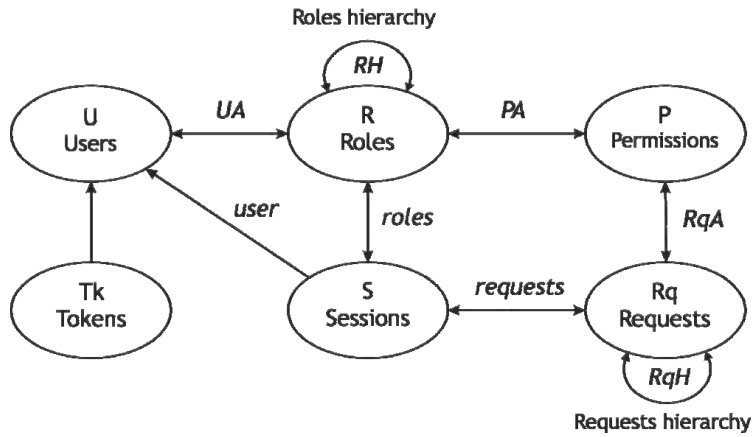
Fig. 2. Elements of path-based RBAC model
