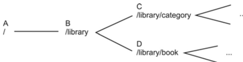
Fig. 1. An example of the inclusion relations on top of requests
