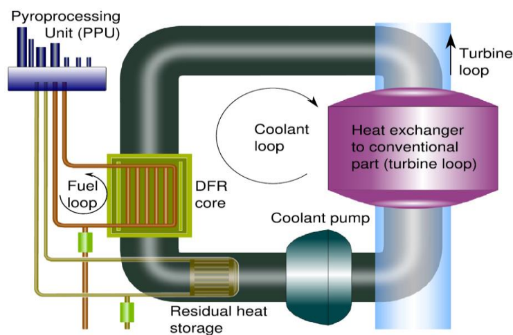
Figure 3. DFR fuel and cooling loop. The fuel circulates between the PPU and the core whereas the coolant loop connects the fissile zone to the conventional part [8].
