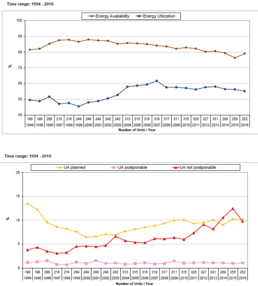
Figure 22. VGB KISSY availability data
