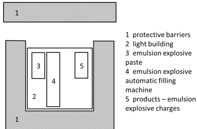
Figure 2. Object for production of emulsion explosive charges (bird's view).
