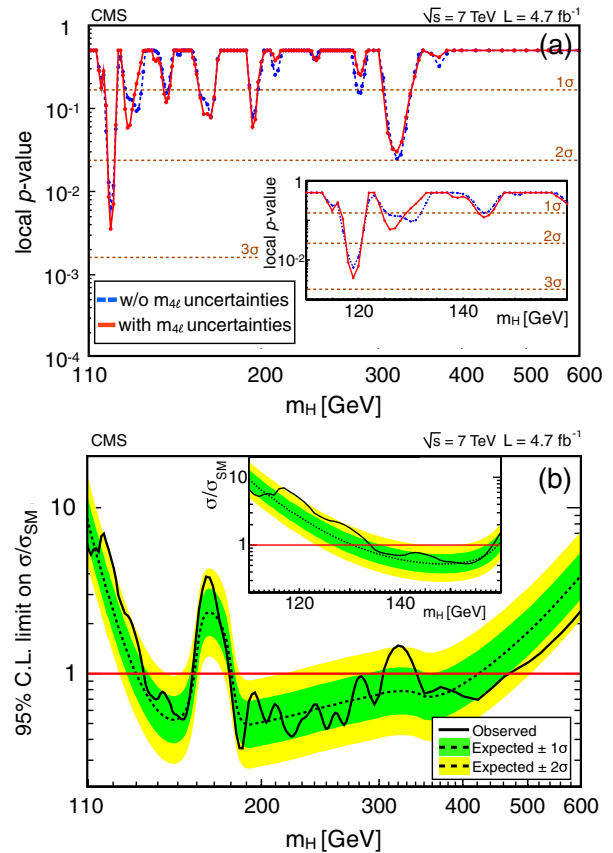
FIG. 2 (color online). (a) The significance of the local excesses with respect to the standard model expectation as a function of the Higgs boson mass, without (blue) or with (red) individual candidate mass measurement uncertainties. (b) The observed and the median expected upper limits at 95% C.L. on \sigma = \sigma(pp \rightarrow H + X) \times \mathcal{B}(H \rightarrow 4\ell) , relative to their standard model prediction \sigma_{SM} , for a Higgs boson in the mass range of 110–600 GeV, using the CL_s approach. The insets expand the low-mass range.
