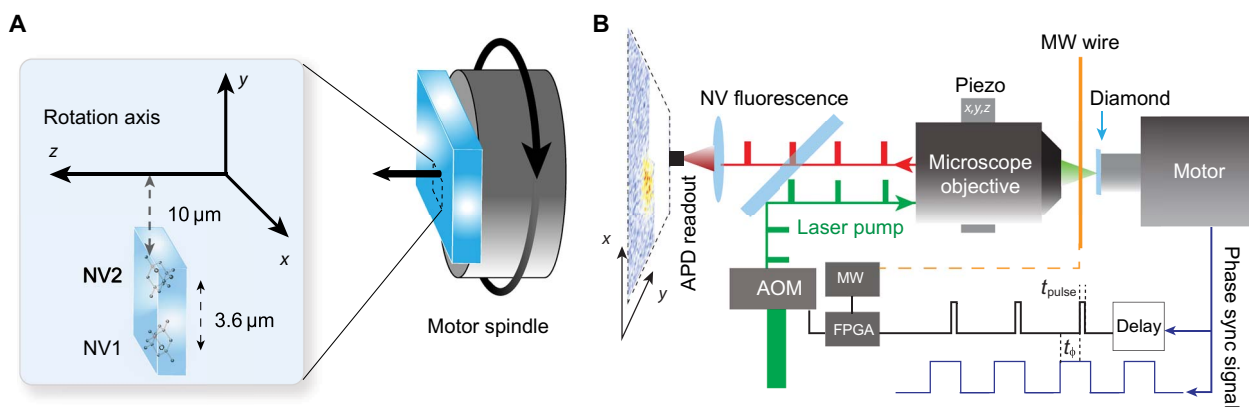
Fig. 1. Experimental schematic and setup. (A) A diamond containing single NV centers is mounted to the spindle of an electric motor that rotates at 3.33 kHz. Two NV centers located 3 \mu\text{m} below the diamond surface, separated by 3.6 \mu\text{m} , and located 10 \mu\text{m} from the center of the rotation axis ( z ) are considered in this work. (B) NV centers are optically prepared and addressed by a scanning confocal microscope: 532-nm excitation light is pulsed for a duration t_{\text{pulse}} synchronously with the motor rotation, and an avalanche photodiode (APD) collects the emitted photons from the NV center. A time delay t_{\text{d}} between the motor synchronization edge and the optical pulse controls the instantaneous angle of the diamond imaged, and a wire located above the surface of the diamond is used to apply microwave (MW) pulses for state manipulation. Current-carrying coils (not shown) are used to apply magnetic fields along the x , y , and z axes. FPGA, field-programmable gate array.
