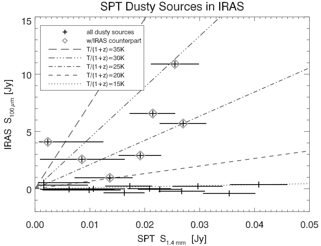
FIG. 11.— IRAS 100 \mu\text{m} flux vs. SPT 1.4 \text{ mm} flux for all SPT dust-dominated sources at S/N > 5 . IRAS flux is taken from a version of the ISSA (Wheelock et al. 1994) 100 \mu\text{m} map which has been filtered to enhance point-source signal-to-noise. Horizontal error bars are the 68% enclosed interval in the posterior 1.4 \text{ mm} flux distribution (as in Table 5). Vertical error bars are the width of the noise distribution in the filtered IRAS map. SPT sources with counterparts within 1 arcmin in the IRAS FSC are shown with diamond symbols. Lines of constant 100 \mu\text{m} – 1.4 \text{ mm} flux ratio are shown for five emission models, all modified blackbody laws with a dust emissivity index of \beta = 1.5 (consistent with the value of \beta used in Dunne & Eales (2001), Chapman et al. (2005), and Kovács et al. (2006)) and with dust temperatures of 15, 20, 25, 30, and 35 K (if the emitter is nearby) or those temperatures times 1+z (if the emitter lies at redshift z ). There is a clear distinction between the locus of sources with IRAS-FSC counterparts — which have flux ratios consistent with warm, low-redshift dust emission — and the points which lie along the x axis and have no counterparts, which must be either at moderate to high redshift or have anomalously cold dust.
