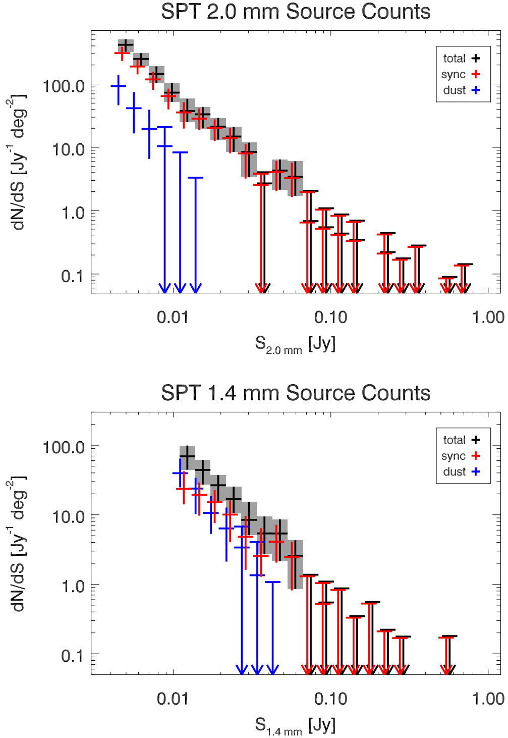
FIG. 9.— Differential source counts by population for the 2.0 mm (upper plot) and 1.4 mm (lower plot) bands. Gray boxes and black crosshairs indicate the total counts in that band. Red crosshairs indicate the synchrotron-dominated population counts and blue crosshairs indicate the dust-dominated counts. Crosshairs with full error bars enclose 68% of the probability about the median and are estimated in the bootstrap over flux described in Sec. 5. Here we have offset the two populations slightly in flux so that they do not lie on top of one another and the total counts are at zero offset. A source is identified as synchrotron-dominated (dust-dominated) if \alpha < 1.66 ( \alpha \geq 1.66 ) in the bootstrap resampling from the joint posterior flux distributions, see Sec. 5. This splits the populations so that their differential counts sum to the total counts. A correction for survey completeness from simulations described in Sec. 3.3 is also applied, and impacts primarily the 1.4 mm counts in the lowest two flux bins.
