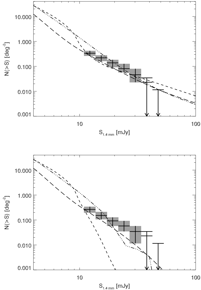
FIG. 12.— Cumulative SPT dust-dominated source counts vs. 1.4 mm flux, with models overplotted. Model curves are as follows: short dashed line : Lagache et al. (2004) 1.38 mm prediction; long dashed line : Negrello et al. (2007) 1.4 mm prediction; dot-dashed line : Pearson & Khan (2009) 1.38 mm prediction. The error regions enclose 68% of the probability centered about the median counts, and are calculated using the bootstrap over the two-band posterior intrinsic flux (at 1.4 mm) that is described in Sec. 5. In these counts, a source is identified as dust-dominated if \alpha \geq 1.66 in the resampling. Top Panel : This plot shows counts and models with all dust-dominated sources included. Bottom Panel : This plot shows counts calculated excluding sources that have IRAS-FSC counterparts (within 1 arcmin) and models calculated excluding populations that should be detectable in the IRAS 60 \mu\text{m} band above the typical FSC limit of 0.2 Jy. The SPT detects sources in excess of what is predicted by the models shown once the IRAS sources have been removed.
