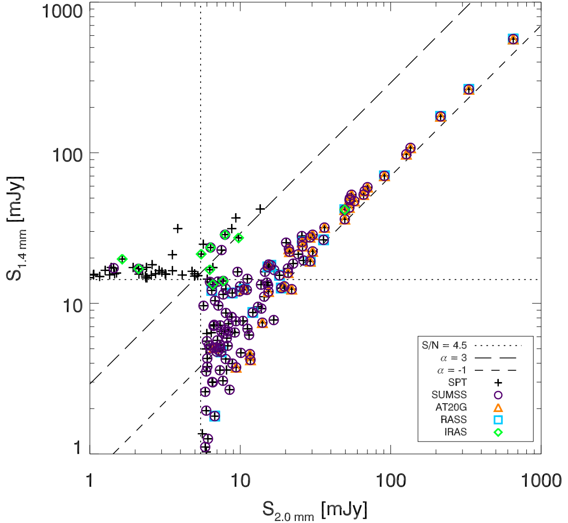
FIG. 7.— Raw 1.4 mm flux versus raw 2.0 mm flux for sources detected above 4.5\sigma (dotted lines) in either band. long-dashed line : A spectral index \alpha = 3 typical for sources dominated by dust emission. short-dashed line : A spectral index \alpha = -1 typical for sources dominated by synchrotron emission. By finding associations within 1 arcmin for SUMSS (purple circles), AT20G (orange triangles), RASS (light blue squares), and IRAS (green diamonds), we see that most synchrotron-dominated sources are previously known. The bright dust-dominated population without counterparts in IRAS is discussed in Sec. 7.2.
