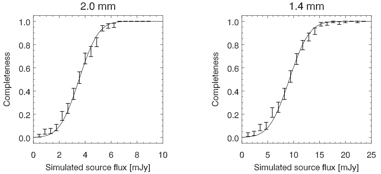
FIG. 5.— The left panel shows the results of the completeness simulation at 2.0 mm; the right panel shows the results of the completeness simulation at 1.4 mm. In each plot, the symbols with error bars show the fraction of sources recovered at > 3\sigma with error bars estimated from binomial statistics. The dashed line shows the best-fit model of the form shown in Eq. 6.
