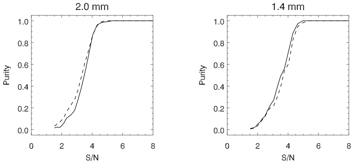
FIG. 6.— Purity in the 2.0 mm-selected sample (left) and the 1.4 mm-selected sample (right). In each plot, the solid line indicates the purity (see Eq. 7) calculated using the inverted map to estimate the number of false detections, while the dashed line indicates the purity calculated using simulated maps to estimate the number of false detections. The situation is more complicated at 2.0 mm than at 1.4 mm due to the presence of SZ (see Sec. 3.3.2 for details).
