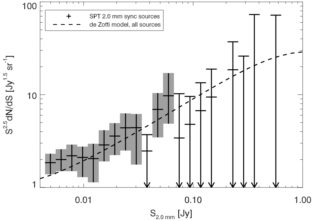
FIG. 10.— Differential counts for the population of sources identified as synchrotron-dominated compared to the De Zotti et al. (2005) model. Here the counts are scaled by S^{2.5} relative to by-band differential counts shown in Fig. 9 to match the (geometrical) convention in AGN literature. The error regions enclose 68% of the probability centered about the median counts, and are calculated using the bootstrap over the two-band posterior intrinsic flux (at 2.0 mm) that is described in Sec. 5. In these counts, a source is identified as synchrotron-dominated if \alpha < 1.66 in the resampling.
