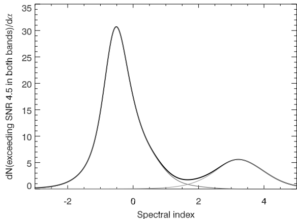
FIG. 8.— The distribution of the posterior spectral indices measured between 1.4 mm and 2.0 mm for sources with signal-to-noise > 4.5 in both bands ( thick black line ). Because we take a flat prior on the spectral index between -3 and 5 (and zero outside), the distribution outside the plotted range here goes to zero. We sum the P(\alpha) for each source (described in Sec. 4.2 and normalize it such that the integral over \alpha is equal to 1 for each source) to give an effective dN/d\alpha for this selection. We then classify the source by the probability that its posterior spectral index distribution exceeds a classification cut, taken here to be \alpha = 1.66 . (This threshold is at the minimum of dN/d\alpha between the two populations.) Sources with > 50\% probability of posterior \alpha > 1.66 are classified as dust dominated and those with < 50\% probability of posterior \alpha > 1.66 are synchrotron-dominated. There are 11 dust sources ( light gray ) and 41 synchrotron sources ( dark gray ) that contribute to this distribution. The population split shown here is robust to changes in the signal-to-noise cut. At lower signal-to-noise cuts, the population features broaden slightly and many sources have poorly-localized P(\alpha) distributions which contribute a floor in dN/d\alpha .
