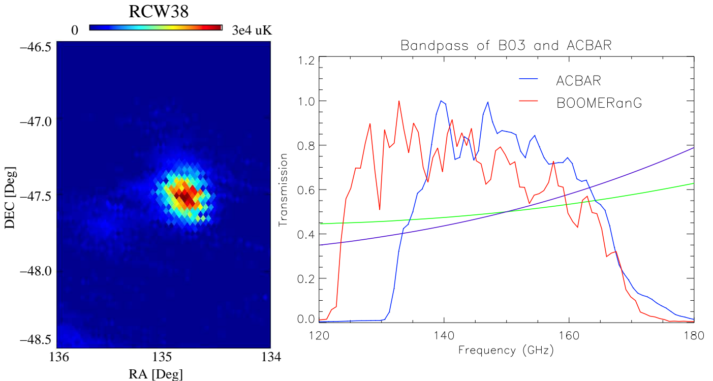
FIG. A9.— On the left-hand side is a map of RCW38 made by B03. The bandpasses for each experiment measured by Fourier transform spectroscopy are shown on the right . The range of possible spectra ( 1\sigma ) for RCW38 is also shown, with each spectrum being normalized to 0.50 at 150 GHz. (green and violet lines).
